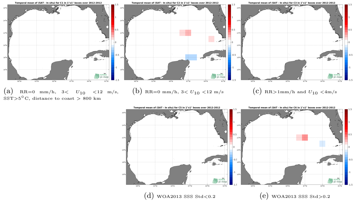
Figure 12: Temporal mean gridded over spatial boxes of size 1^\circ \times 1^\circ of \Delta SSS (CCI SSS L4 Merged-OI v2.31 - 30-day running (ESA) - TSG (GOSUD-Sailing-ship)) for 5 different subdatasets corresponding to: RR=0 mm/h, 3 < U_{10} < 12 m/s, SST >5^\circ\text{C} , distance to coast > 800 km (a), RR=0 mm/h, 3 < U_{10} < 12 m/s (b), RR >1 mm/h and U_{10} < 4 m/s (c), WOA2013 SSS Std <0.2 (d), WOA2013 SSS Std >0.2 (e).
