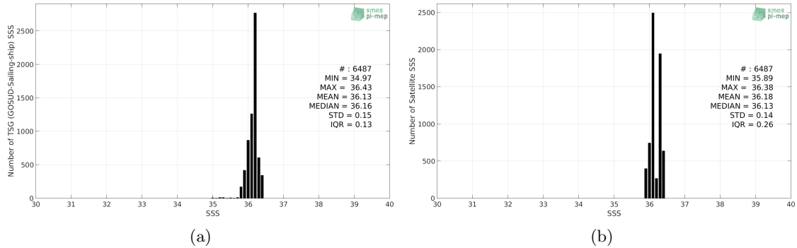
Figure 2: Histograms of SSS from TSG (GOSUD-Sailing-ship) (a) and CCI SSS L4 Merged-OI v2.31 - 30-day running (ESA) (b) considering all match-up pairs per bins of 0.1 over the Gulf of Mexico Pi-MEP region and for the full satellite product period.
