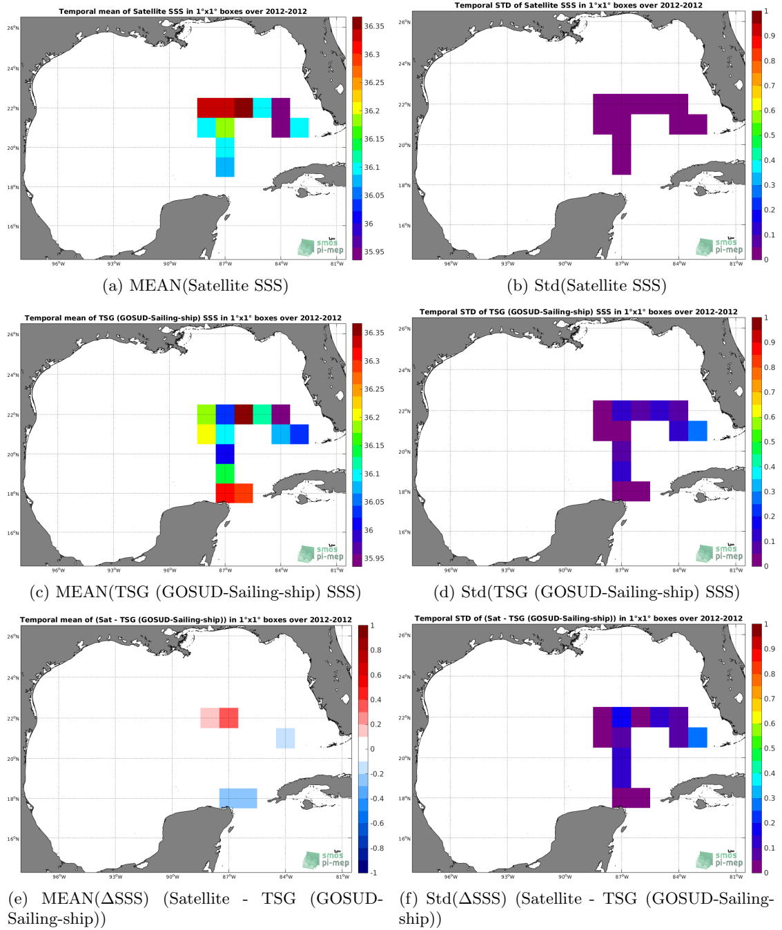
Figure 6: Temporal mean (left) and Std (right) of SSS from CCI L4 Merged-OI v2.31 - 30-day running (ESA) (top), TSG (GOSUD-Sailing-ship) (middle), and of \Delta SSS (Satellite - TSG (GOSUD-Sailing-ship)). Only match-up pairs are used to generate these maps.
