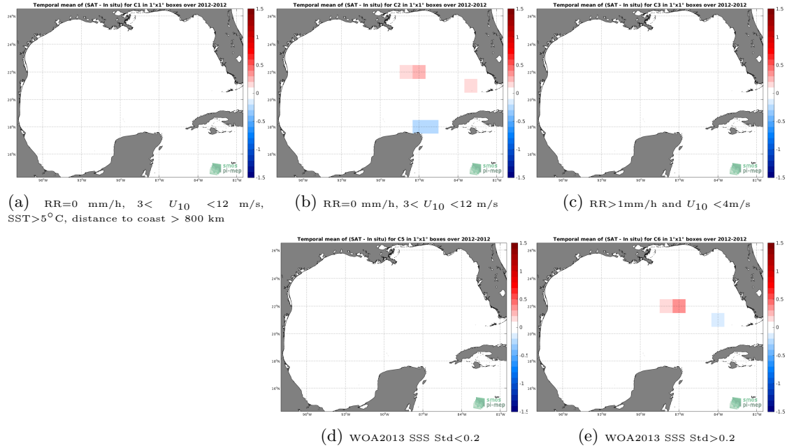
Figure 12: Temporal mean gridded over spatial boxes of size 1^{\circ}\times 1^{\circ} of \Delta SSS (CCI L4 Merged-OI v2.31 - 30-day running (ESA) - TSG (GOSUD-Sailing-ship)) for 5 different subdatasets corresponding to:RR=0 mm/h, 3 < U_{10} < 12 m/s, SST >5^{\circ}\text{C} , distance to coast > 800 km (a), RR=0 mm/h, 3 < U_{10} < 12 m/s (b), RR >1 mm/h and U_{10} < 4 m/s (c), WOA2013 SSS Std <0.2 (d), WOA2013 SSS Std >0.2 (e).
