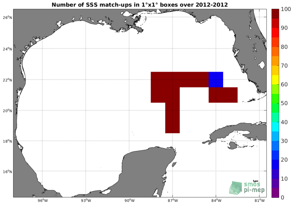
Figure 4: Number of SSS match-ups between TSG (GOSUD-Sailing-ship) SSS and the CCI L4 Merged-OI v2.31 - 30-day running (ESA) SSS product for the Gulf of Mexico Pi-MEP region over 1^\circ \times 1^\circ boxes and for the full satellite product period.
