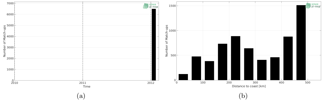
Figure 1: Number of match-ups between TSG (GOSUD-Sailing-ship) and CCI L4 Merged-OI v2.31 - 30-day running (ESA) SSS as a function of time (a) and as function of the distance to coast (b) over the Gulf of Mexico Pi-MEP region and for the full satellite product period.
