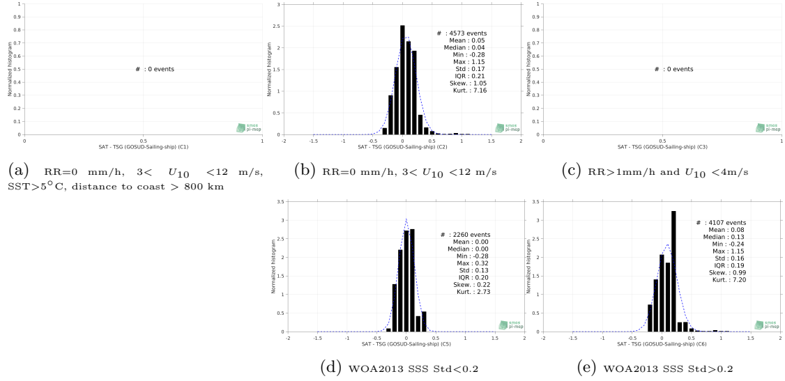
Figure 13: Normalized histogram of \Delta\text{SSS} (CCI L4 Merged-OI v2.31 - 30-day running (ESA) - TSG (GOSUD-Sailing-ship)) for 5 different subdatasets corresponding to: RR=0 mm/h, 3 < U_{10} < 12 m/s, SST > 5^\circ\text{C} , distance to coast > 800 km (a), RR=0 mm/h, 3 < U_{10} < 12 m/s (b), RR > 1\text{mm/h} and U_{10} < 4\text{m/s} (c), WOA2013 SSS Std <0.2 (d), WOA2013 SSS Std >0.2 (e).
