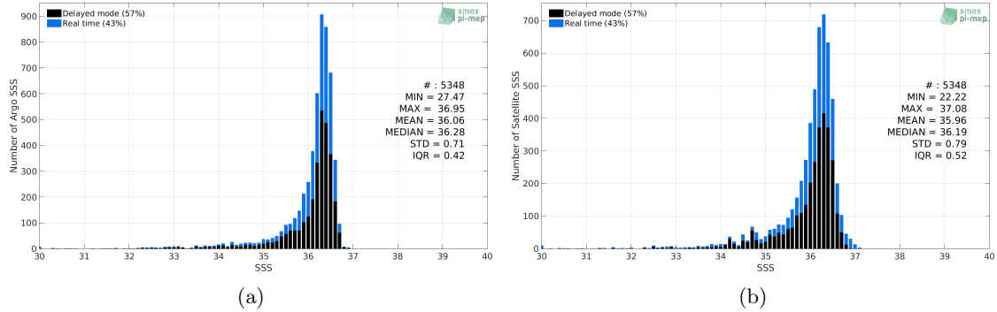
Figure 2: Histograms of SSS from Argo (a) and CCI SSS L4 Merged-OI v2.31 - 30-day running (ESA) (b) considering all match-up pairs per bins of 0.1 over the Gulf of Mexico Pi-MEP region and for the full satellite product period.
