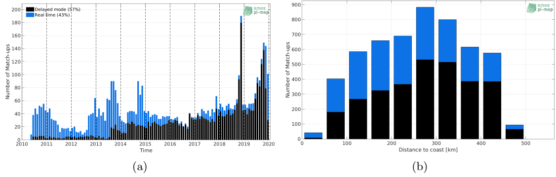
Figure 1: Number of match-ups between Argo and CCI SSS L4 Merged-OI v2.31 - 30-day running (ESA) SSS as a function of time (a) and as function of the distance to coast (b) over the Gulf of Mexico Pi-MEP region and for the full satellite product period.
