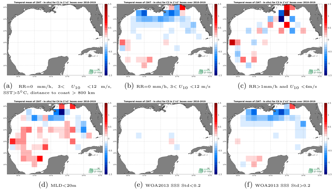
Figure 12: Temporal mean gridded over spatial boxes of size 1^\circ \times 1^\circ of \Delta SSS (CCI SSS L4 Merged-OI v2.31 - 30-day running (ESA) - Argo) for 6 different subdatasets corresponding to: RR=0 mm/h, 3 < U_{10} < 12 m/s, SST >5^\circ\text{C} , distance to coast > 800 km (a), RR=0 mm/h, 3 < U_{10} < 12 m/s (b), RR >1 mm/h and U_{10} < 4 m/s (c),MLD <20 m (d),WOA2013 SSS Std <0.2 (e),WOA2013 SSS Std >0.2 (f).
