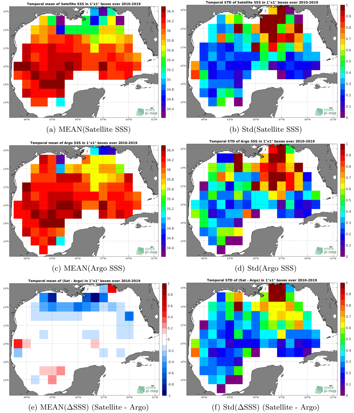
Figure 6: Temporal mean (left) and Std (right) of SSS from CCI SSS L4 Merged-OI v2.31 - 30-day running (ESA) (top), Argo (middle), and of \Delta SSS (Satellite - Argo). Only match-up pairs are used to generate these maps.
