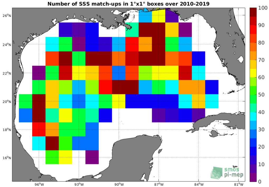
Figure 4: Number of SSS match-ups between Argo SSS and the CCI SSS L4 Merged-OI v2.31 - 30-day running (ESA) SSS product for the Gulf of Mexico Pi-MEP region over 1^\circ \times 1^\circ boxes and for the full satellite product period.
