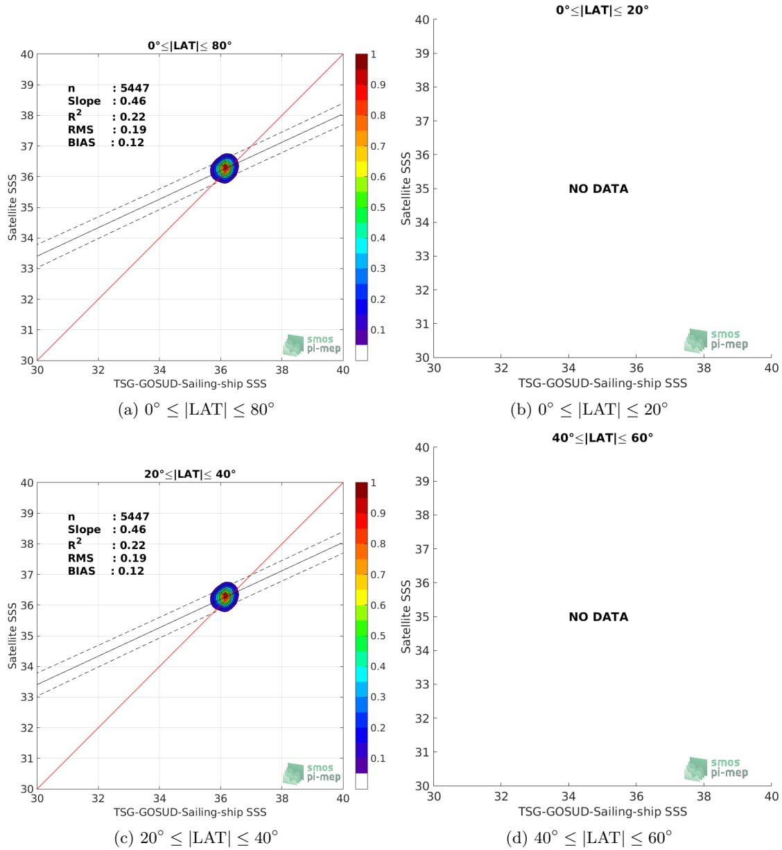
Figure 9: Contour maps of the concentration of CCI-L4-ESA-MERGED-OI-V1.8-7DAY-RUNNING SSS (y-axis) versus TSG-GOSUD-Sailing-ship SSS (x-axis) at match-up pairs for different latitude bands. For each plot, the red line shows x=y . The black thin and dashed lines indicate a linear fit through the data cloud and the \pm 95\% confidence levels, respectively. The number match-up pairs n , the slope and R^2 coefficient of the linear fit, the root mean square (RMS) and the mean bias between satellite and in situ data are indicated for each latitude band in each plots.
