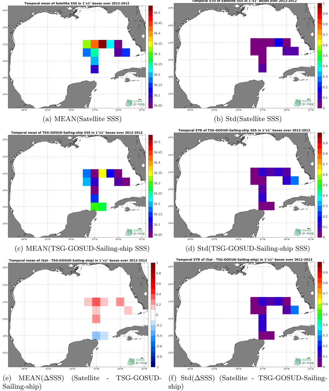
Figure 6: Temporal mean (left) and Std (right) of SSS from CCI-L4-ESA-MERGED-OI-V1.8-7DAY-RUNNING (top), TSG-GOSUD-Sailing-ship (middle), and of \Delta SSS (Satellite - TSG-GOSUD-Sailing-ship). Only match-up pairs are used to generate these maps.
