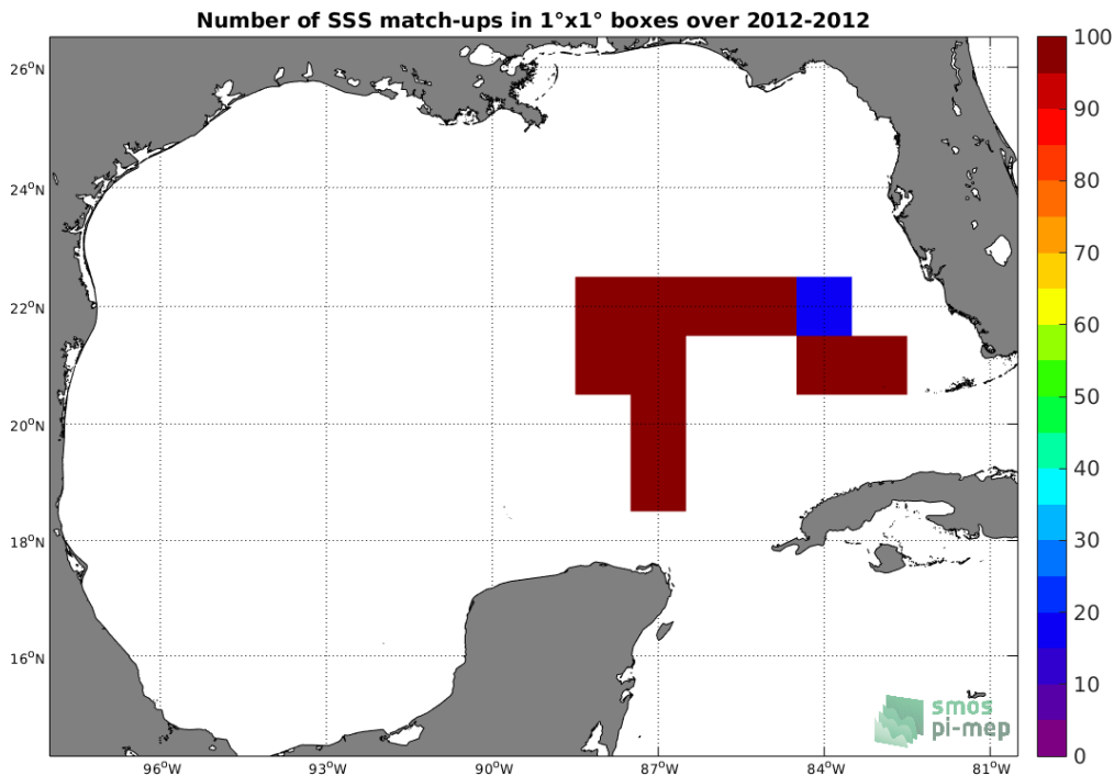
Figure 4: Number of SSS match-ups between TSG-GOSUD-Sailing-ship SSS and the CCI-L4-ESA-MERGED-OI-V1.8-7DAY-RUNNING SSS product for the Gulf of Mexico Pi-MEP region over 1°x1° boxes and for the full satellite product period.
