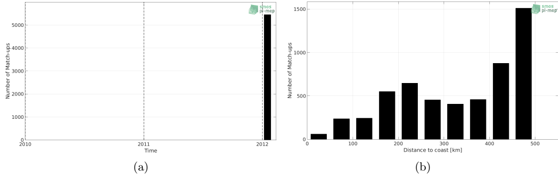
Figure 1: Number of match-ups between TSG-GOSUD-Sailing-ship and CCI-L4-ESA-MERGED-OI-V1.8-7DAY-RUNNING SSS as a function of time (a) and as function of the distance to coast (b) over the Gulf of Mexico Pi-MEP region and for the full satellite product period.
