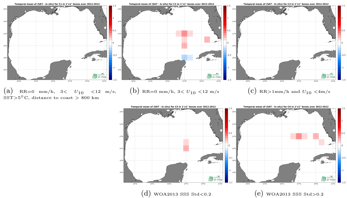
Figure 12: Temporal mean gridded over spatial boxes of size 1^\circ \times 1^\circ of \Delta SSS (CCI-L4-ESA-MERGED-OI-V1.8-7DAY-RUNNING - TSG-GOSUD-Sailing-ship) for 5 different subdatasets corresponding to:RR=0 mm/h, 3 < U_{10} < 12 m/s, SST >5^\circ\text{C} , distance to coast > 800 km (a), RR=0 mm/h, 3 < U_{10} < 12 m/s (b), RR >1 mm/h and U_{10} < 4 m/s (c), WOA2013 SSS Std <0.2 (d), WOA2013 SSS Std >0.2 (e).
