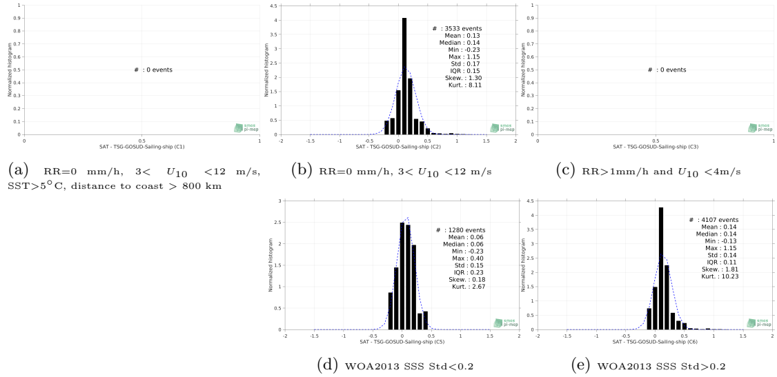
Figure 13: Normalized histogram of \Delta SSS (CCI-L4-ESA-MERGED-OI-V1.8-7DAY-RUNNING - TSG-GOSUD-Sailing-ship) for 5 different subdatasets corresponding to: RR=0 mm/h, 3 < U_{10} < 12 m/s, SST > 5°C, distance to coast > 800 km (a), RR=0 mm/h, 3 < U_{10} < 12 m/s (b), RR > 1mm/h and U_{10} < 4 m/s (c), WOA2013 SSS Std < 0.2 (d), WOA2013 SSS Std > 0.2 (e).
