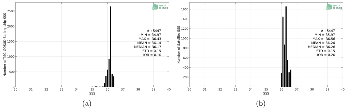
Figure 2: Histograms of SSS from TSG-GOSUD-Sailing-ship (a) and CCI-L4-ESA-MERGED-OI-V1.8-7DAY-RUNNING (b) considering all match-up pairs per bins of 0.1 over the Gulf of Mexico Pi-MEP region and for the full satellite product period.
