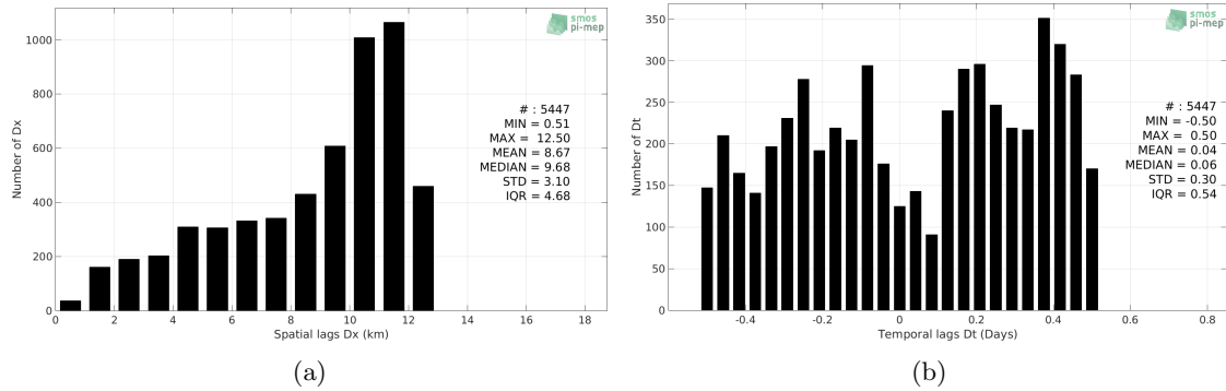
Figure 5: Histograms of the spatial (a) and temporal (b) lags between the time of the TSG-GOSUD-Sailing-ship measurements and the date of the corresponding CCI-L4-ESA-MERGED-OI-V1.8-7DAY-RUNNING SSS product.
