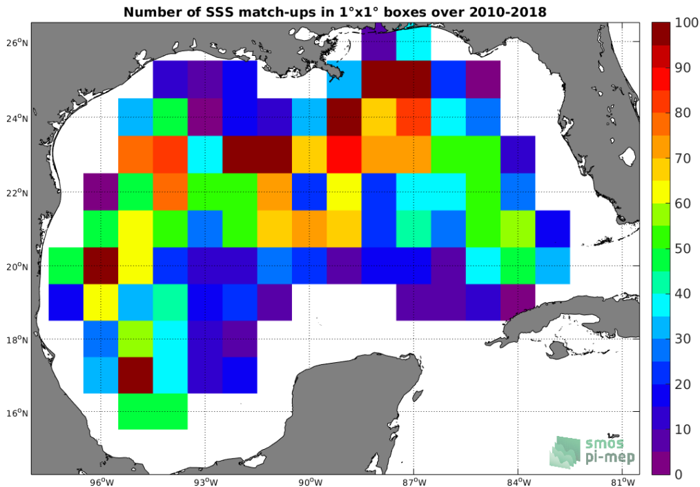
Figure 4: Number of SSS match-ups between Argo SSS and the CCI-L4-ESA-MERGED-OI-V1.8-30DAY-RUNNING SSS product for the Gulf of Mexico Pi-MEP region over 1°x1° boxes and for the full satellite product period.
