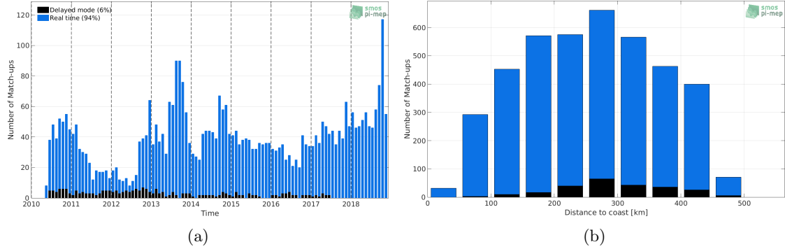
Figure 1: Number of match-ups between Argo and CCI-L4-ESA-MERGED-OI-V1.8-30DAY-RUNNING SSS as a function of time (a) and as function of the distance to coast (b) over the Gulf of Mexico Pi-MEP region and for the full satellite product period.
