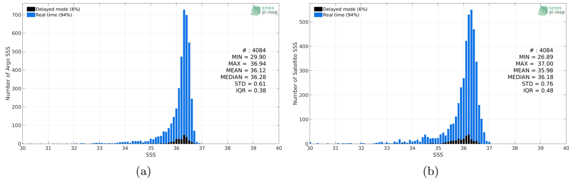
Figure 2: Histograms of SSS from Argo (a) and CCI-L4-ESA-MERGED-OI-V1.8-30DAY-RUNNING (b) considering all match-up pairs per bins of 0.1 over the Gulf of Mexico Pi-MEP region and for the full satellite product period.
