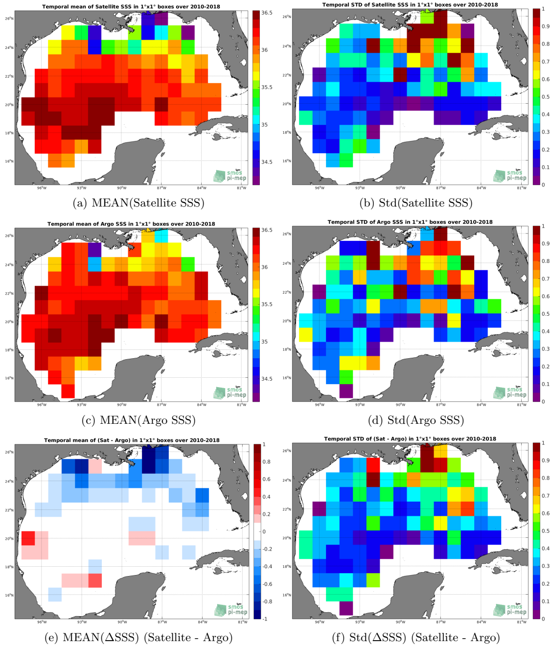
Figure 6: Temporal mean (left) and Std (right) of SSS from CCI-L4-ESA-MERGED-OI-V1.8-30DAY-RUNNING (top), Argo (middle), and of \Delta SSS (Satellite - Argo). Only match-up pairs are used to generate these maps.
