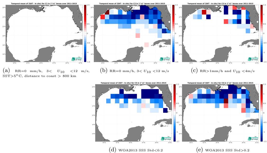
Figure 14: Temporal mean gridded over spatial boxes of size 1^\circ \times 1^\circ of \Delta SSS (Aquarius SSS L4 OI v5 - Weekly (IPRC) - TSG (SAMOS)) for 5 different subdatasets corresponding to:RR=0 mm/h, 3 < U_{10} < 12 m/s, SST > 5^\circ\text{C} , distance to coast > 800 km (a), RR=0 mm/h, 3 < U_{10} < 12 m/s (b), RR > 1 mm/h and U_{10} < 4 m/s (c), WOA2013 SSS Std < 0.2 (d), WOA2013 SSS Std > 0.2 (e).
