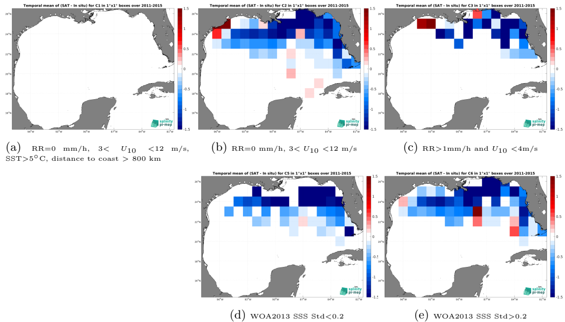
Figure 12: Temporal mean gridded over spatial boxes of size 1^{\circ}\times 1^{\circ} of \Delta\text{SSS} (Aquarius SSS L4 OI v5 - Weekly (IPRC) - TSG (SAMOS)) for 5 different subdatasets corresponding to:RR=0 mm/h, 3 < U_{10} < 12 m/s, SST >5^{\circ}\text{C} , distance to coast > 800 km (a), RR=0 mm/h, 3 < U_{10} < 12 m/s (b), RR >1 mm/h and U_{10} < 4 m/s (c), WOA2013 SSS Std <0.2 (d), WOA2013 SSS Std >0.2 (e).
