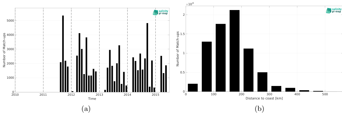
Figure 1: Number of match-ups between TSG (SAMOS) and Aquarius SSS L4 OI v5 - Weekly (IPRC) SSS as a function of time (a) and as function of the distance to coast (b) over the Gulf of Mexico Pi-MEP region and for the full satellite product period.
