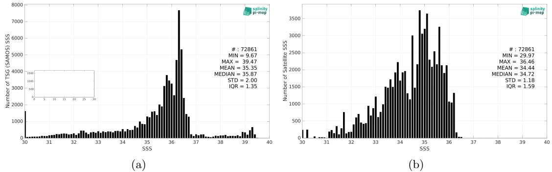
Figure 2: Histograms of SSS from TSG (SAMOS) (a) and Aquarius SSS L4 OI v5 - Weekly (IPRC) (b) considering all match-up pairs per bins of 0.1 over the Gulf of Mexico Pi-MEP region and for the full satellite product period.
