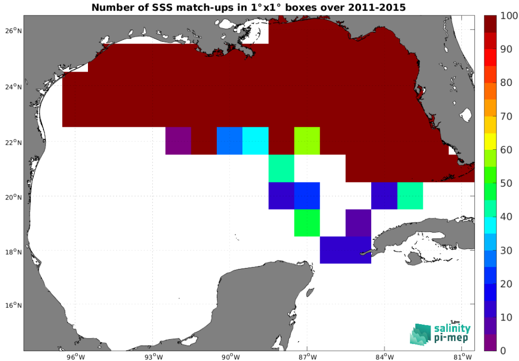
Figure 4: Number of SSS match-ups between TSG (SAMOS) SSS and the Aquarius SSS L4 OI v5 - Weekly (IPRC) SSS product for the Gulf of Mexico Pi-MEP region over 1^\circ \times 1^\circ boxes and for the full satellite product period.
