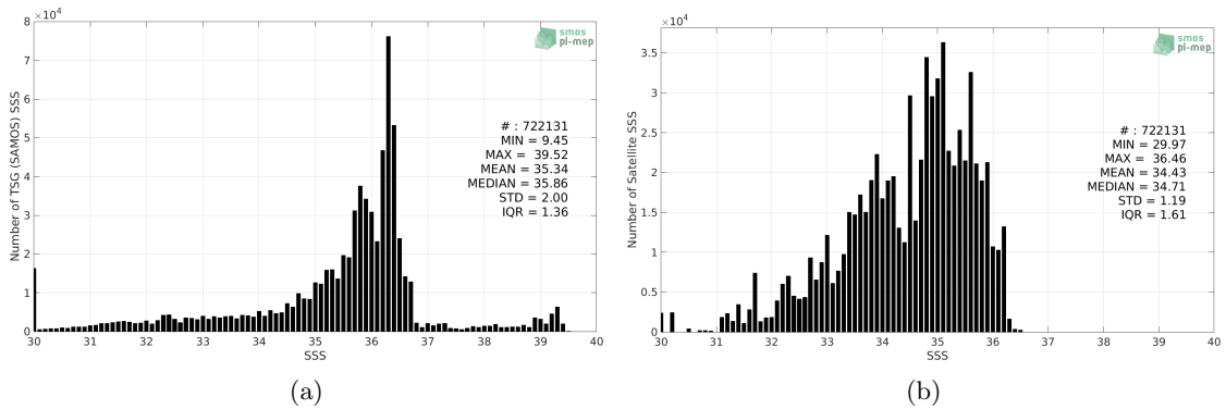
Figure 2: Histograms of SSS from TSG (SAMOS) (a) and Aquarius SSS L4 OI v5 - Weekly (IPRC) (b) considering all match-up pairs per bins of 0.1 over the Gulf of Mexico Pi-MEP region and for the full satellite product period.
