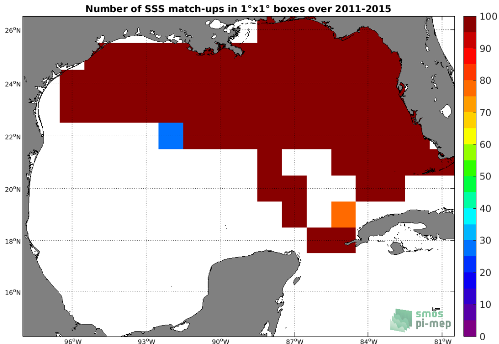
Figure 4: Number of SSS match-ups between TSG (SAMOS) SSS and the Aquarius SSS L4 OI v5 - Weekly (IPRC) SSS product for the Gulf of Mexico Pi-MEP region over 1°x1° boxes and for the full satellite product period.
