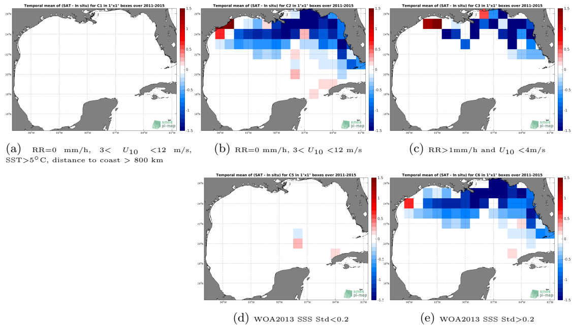
Figure 12: Temporal mean gridded over spatial boxes of size 1^{\circ}\times 1^{\circ} of \Delta\text{SSS} (Aquarius-L4-IPRC-V5-WEEKLY - TSG-SAMOS) for 5 different subdatasets corresponding to:RR=0 mm/h, 3 < U_{10} < 12 m/s, SST >5^{\circ}\text{C} , distance to coast > 800 km (a), RR=0 mm/h, 3 < U_{10} < 12 m/s (b), RR >1 mm/h and U_{10} < 4 m/s (c), WOA2013 SSS Std <0.2 (d), WOA2013 SSS Std >0.2 (e).
