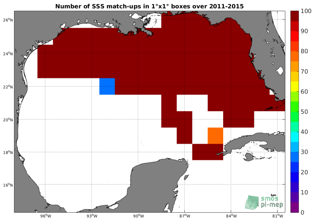
Figure 4: Number of SSS match-ups between TSG-SAMOS SSS and the Aquarius-L4-IPRC-V5-WEEKLY SSS product for the Gulf of Mexico Pi-MEP region over 1°x1° boxes and for the full satellite product period.
