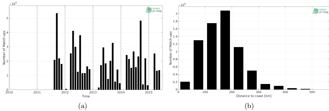
Figure 1: Number of match-ups between TSG-SAMOS and Aquarius-L4-IPRC-V5-WEEKLY SSS as a function of time (a) and as function of the distance to coast (b) over the Gulf of Mexico Pi-MEP region and for the full satellite product period.
