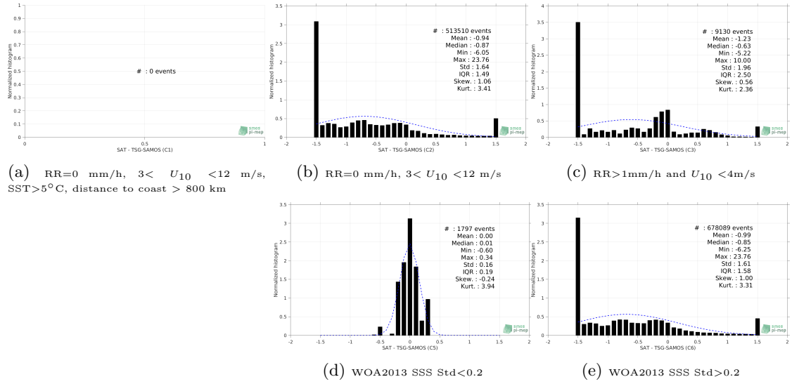
Figure 13: Normalized histogram of \Delta SSS (Aquarius-L4-IPRC-V5-WEEKLY - TSG-SAMOS) for 5 different subdatasets corresponding to: RR=0 mm/h, 3 < U_{10} < 12 m/s, SST>5°C, distance to coast > 800 km (a), RR=0 mm/h, 3 < U_{10} < 12 m/s (b), RR>1mm/h and U_{10} < 4 m/s (c), WOA2013 SSS Std<0.2 (d), WOA2013 SSS Std>0.2 (e).
