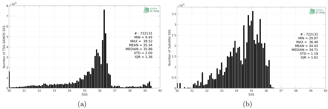
Figure 2: Histograms of SSS from TSG-SAMOS (a) and Aquarius-L4-IPRC-V5-WEEKLY (b) considering all match-up pairs per bins of 0.1 over the Gulf of Mexico Pi-MEP region and for the full satellite product period.
