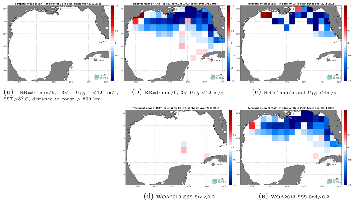
Figure 12: Temporal mean gridded over spatial boxes of size 1^\circ \times 1^\circ of \Delta SSS (Aquarius-L4-IPRC-V5-WEEKLY - TSG-SAMOS) for 5 different subdatasets corresponding to:RR=0 mm/h, 3 < U_{10} < 12 m/s, SST >5^\circ\text{C} , distance to coast > 800 km (a), RR=0 mm/h, 3 < U_{10} < 12 m/s (b), RR >1 mm/h and U_{10} < 4 m/s (c), WOA2013 SSS Std <0.2 (d), WOA2013 SSS Std >0.2 (e).
