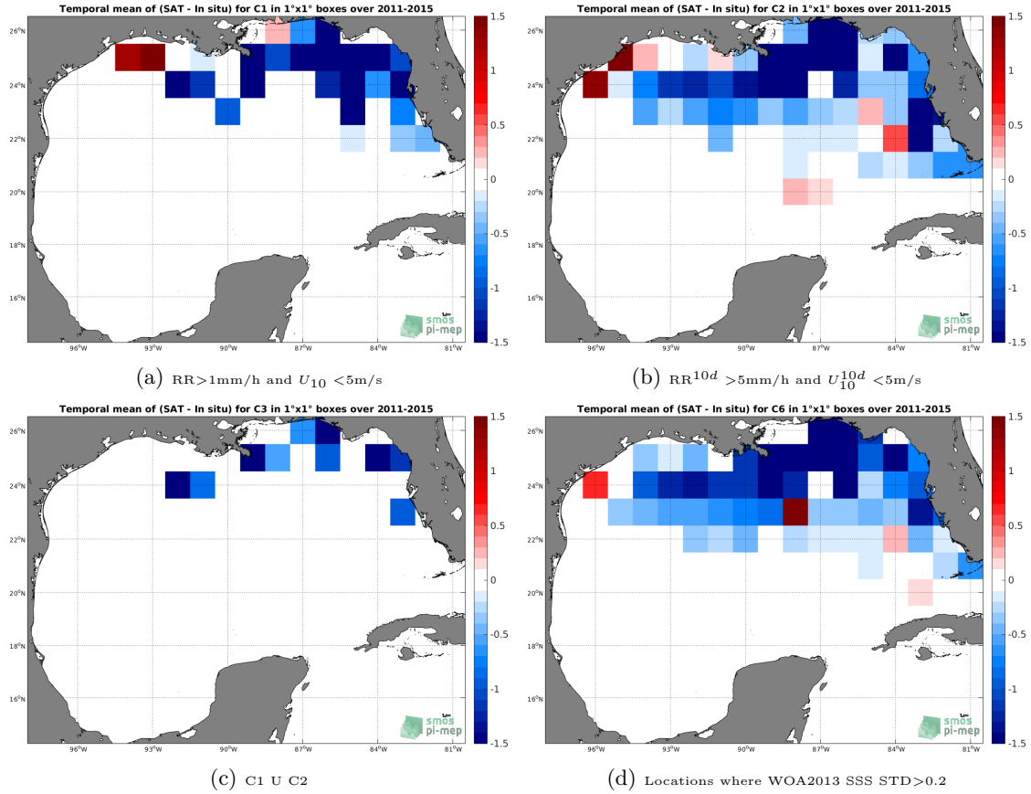
Figure 12: Temporal mean gridded over spatial boxes of size 1^\circ \times 1^\circ of \Delta SSS (Aquarius-L4-IPRC-V5-WEEKLY - TSG-SAMOS) for 4 different subdatasets corresponding to: RR > 1\text{mm/h} and U_{10} < 5\text{m/s} (a), RR^{10d} > 5\text{mm/h} and U_{10}^{10d} < 5\text{m/s} (b), C1 U C2 (c), Locations where WOA2013 SSS STD > 0.2 (d).
