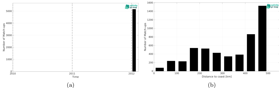
Figure 2: Number of match-ups between TSG (GOSUD-Sailing-ship) and Aquarius SSS L4 OI v5 - Weekly (IPRC) SSS as a function of time (a) and as function of the distance to coast (b) over the Gulf of Mexico Pi-MEP region and for the full satellite product period.
