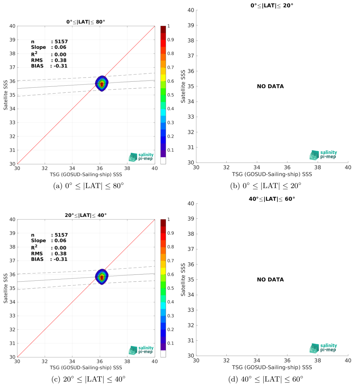
Figure 10: Contour maps of the concentration of Aquarius SSS L4 OI v5 - Weekly (IPRC) SSS (y-axis) versus TSG (GOSUD-Sailing-ship) SSS (x-axis) at match-up pairs for different latitude bands. For each plot, the red line shows x=y . The black thin and dashed lines indicate a linear fit through the data cloud and the \pm 95\% confidence levels, respectively. The number match-up pairs n , the slope and R^2 coefficient of the linear fit, the root mean square (RMS) and the mean bias between satellite and in situ data are indicated for each latitude band in each plots.
