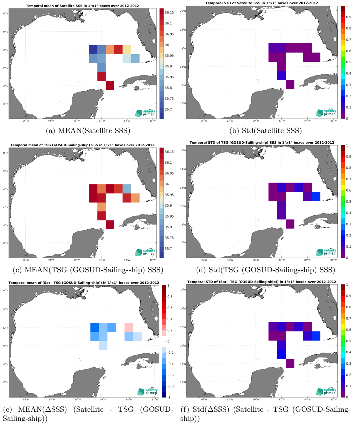
Figure 7: Temporal mean (left) and Std (right) of SSS from Aquarius SSS L4 OI v5 - Weekly (IPRC) (top), TSG (GOSUD-Sailing-ship) (middle), and of \Delta SSS (Satellite - TSG (GOSUD-Sailing-ship)). Only match-up pairs are used to generate these maps.
