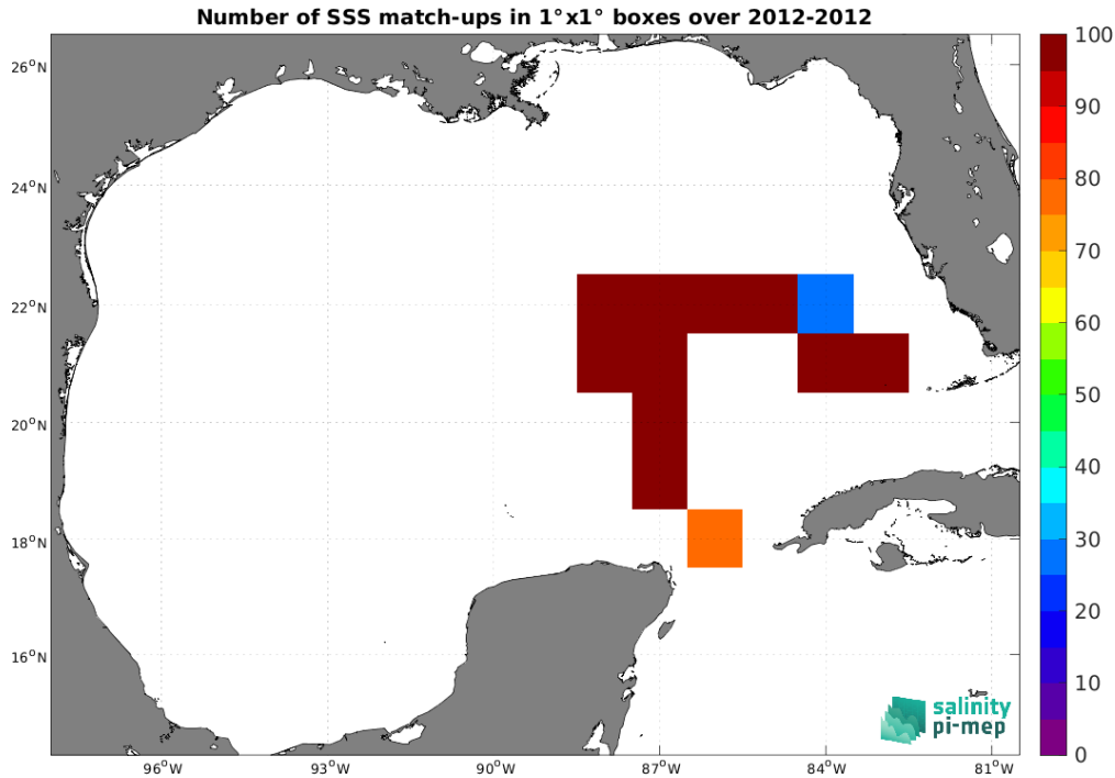
Figure 5: Number of SSS match-ups between TSG (GOSUD-Sailing-ship) SSS and the Aquarius SSS L4 OI v5 - Weekly (IPRC) SSS product for the Gulf of Mexico Pi-MEP region over 1^\circ \times 1^\circ boxes and for the full satellite product period.
