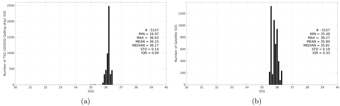
Figure 3: Histograms of SSS from TSG (GOSUD-Sailing-ship) (a) and Aquarius SSS L4 OI v5 - Weekly (IPRC) (b) considering all match-up pairs per bins of 0.1 over the Gulf of Mexico Pi-MEP region and for the full satellite product period.
