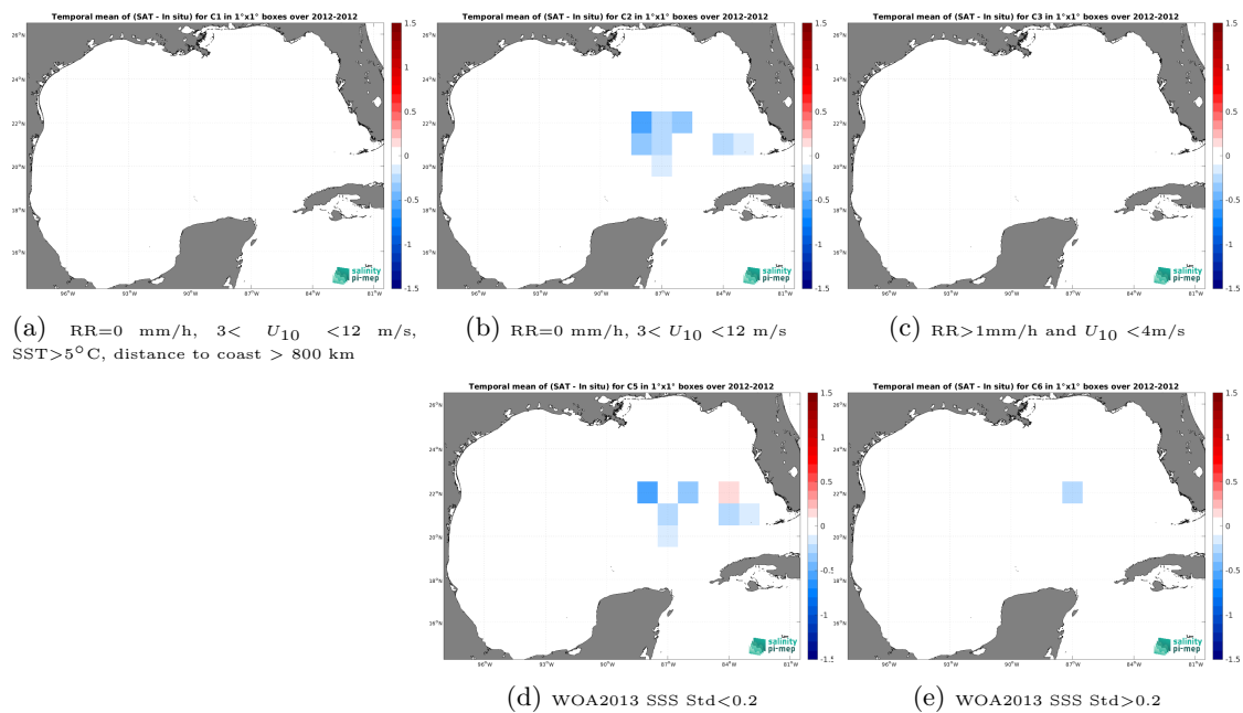
Figure 14: Temporal mean gridded over spatial boxes of size 1^\circ \times 1^\circ of \Delta SSS (Aquarius SSS L4 OI v5 - Weekly (IPRC) - TSG (GOSUD-Sailing-ship)) for 5 different subdatasets corresponding to:RR=0 mm/h, 3 < U_{10} < 12 m/s, SST>5°C, distance to coast > 800 km (a), RR=0 mm/h, 3 < U_{10} < 12 m/s (b), RR>1mm/h and U_{10} < 4 m/s (c), WOA2013 SSS Std<0.2 (d), WOA2013 SSS Std>0.2 (e).
