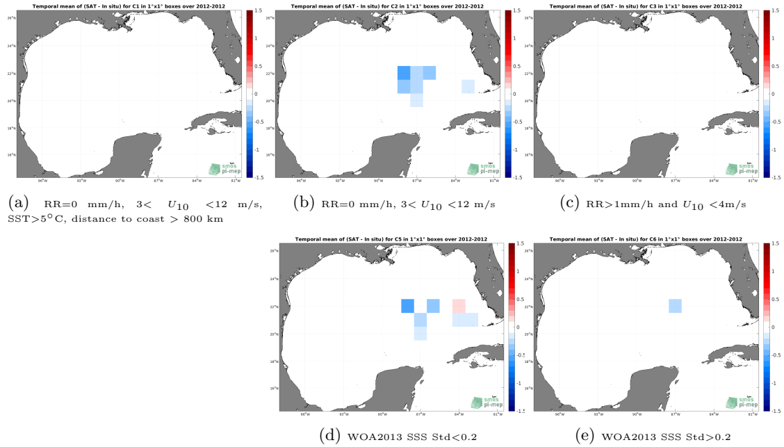
Figure 12: Temporal mean gridded over spatial boxes of size 1^{\circ}\times 1^{\circ} of \Delta SSS (Aquarius SSS L4 OI v5 - Weekly (IPRC) - TSG (GOSUD-Sailing-ship)) for 5 different subdatasets corresponding to:RR=0 mm/h, 3 < U_{10} < 12 m/s, SST >5^{\circ}\text{C} , distance to coast > 800 km (a), RR=0 mm/h, 3 < U_{10} < 12 m/s (b), RR >1 mm/h and U_{10} < 4 m/s (c), WOA2013 SSS Std <0.2 (d), WOA2013 SSS Std >0.2 (e).
