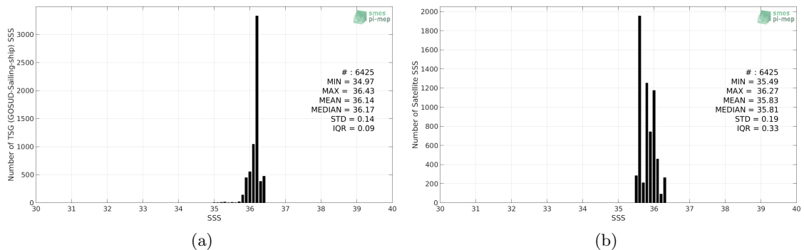
Figure 2: Histograms of SSS from TSG (GOSUD-Sailing-ship) (a) and Aquarius SSS L4 OI v5 - Weekly (IPRC) (b) considering all match-up pairs per bins of 0.1 over the Gulf of Mexico Pi-MEP region and for the full satellite product period.
