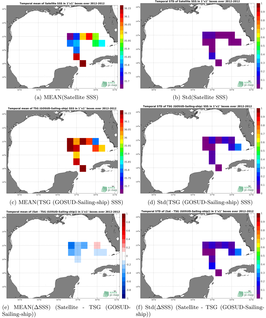
Figure 6: Temporal mean (left) and Std (right) of SSS from Aquarius SSS L4 OI v5 - Weekly (IPRC) (top), TSG (GOSUD-Sailing-ship) (middle), and of \Delta SSS (Satellite - TSG (GOSUD-Sailing-ship)). Only match-up pairs are used to generate these maps.
