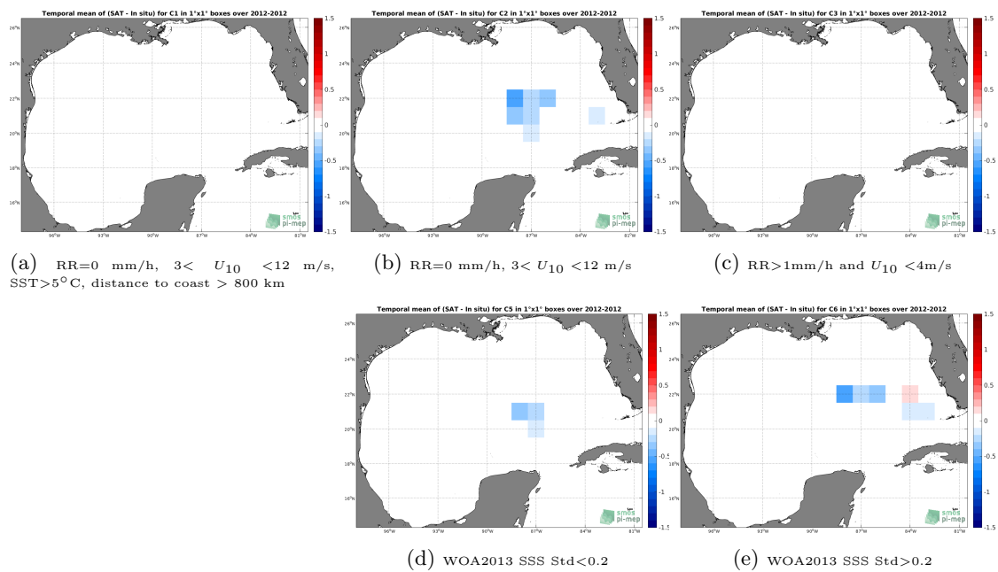
Figure 12: Temporal mean gridded over spatial boxes of size 1^\circ \times 1^\circ of \Delta SSS (Aquarius-L4-IPRC-V5-WEEKLY - TSG-GOSUD-Sailing-ship) for 5 different subdatasets corresponding to:RR=0 mm/h, 3 < U_{10} < 12 m/s, SST > 5^\circ\text{C} , distance to coast > 800 km (a), RR=0 mm/h, 3 < U_{10} < 12 m/s (b), RR > 1 mm/h and U_{10} < 4 m/s (c), WOA2013 SSS Std < 0.2 (d), WOA2013 SSS Std > 0.2 (e).
