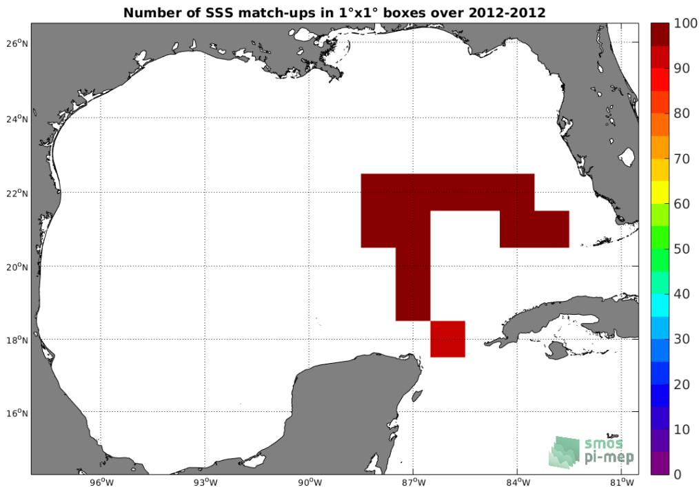
Figure 4: Number of SSS match-ups between TSG-GOSUD-Sailing-ship SSS and the Aquarius-L4-IPRC-V5-WEEKLY SSS product for the Gulf of Mexico Pi-MEP region over 1^\circ \times 1^\circ boxes and for the full satellite product period.
