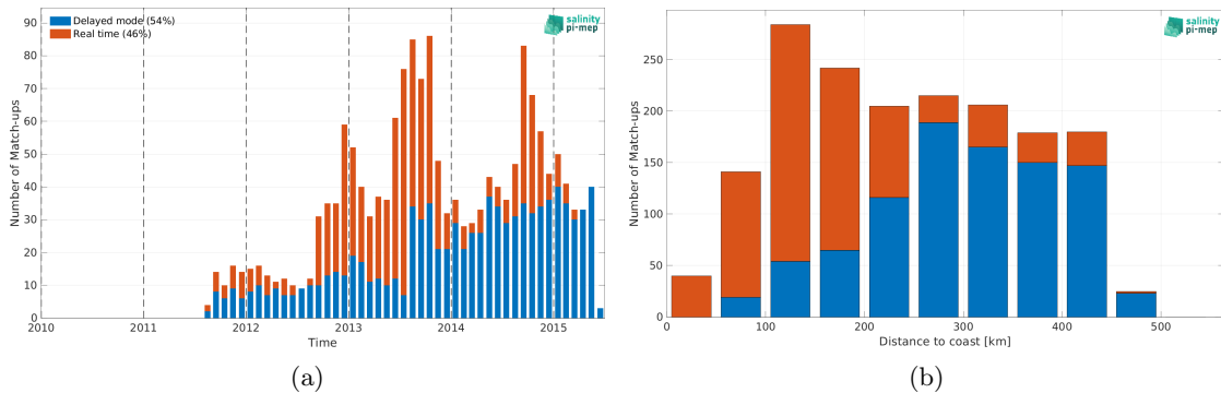
Figure 2: Number of match-ups between Argo and Aquarius SSS L4 OI v5 - Weekly (IPRC) SSS as a function of time (a) and as function of the distance to coast (b) over the Gulf of Mexico Pi-MEP region and for the full satellite product period.
