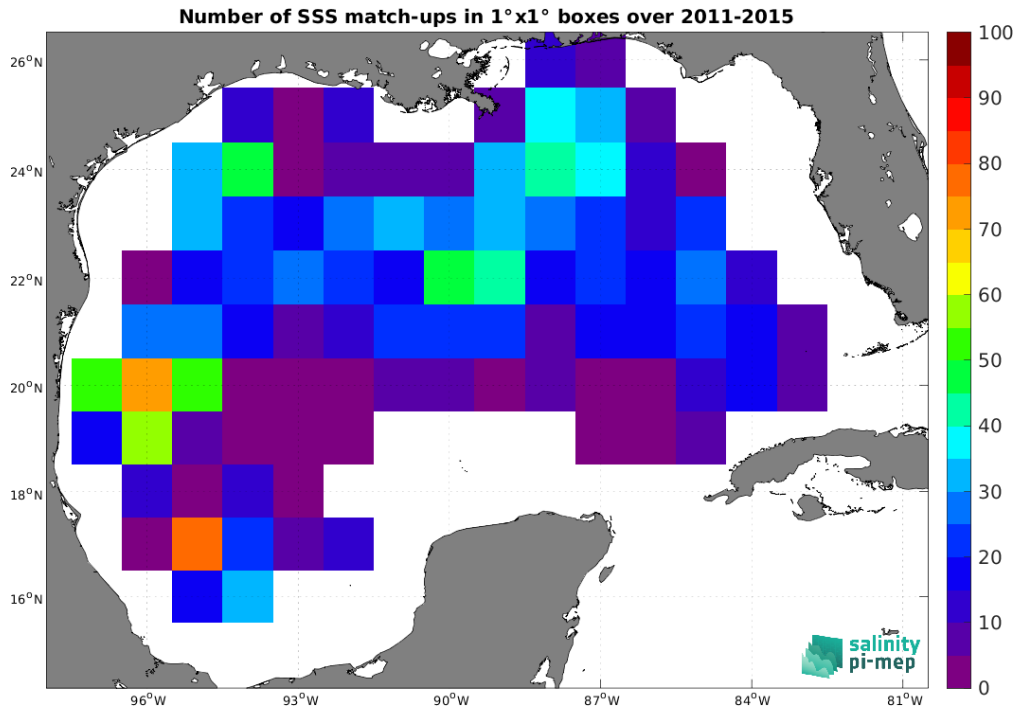
Figure 5: Number of SSS match-ups between Argo SSS and the Aquarius SSS L4 OI v5 - Weekly (IPRC) SSS product for the Gulf of Mexico Pi-MEP region over 1^\circ \times 1^\circ boxes and for the full satellite product period.
