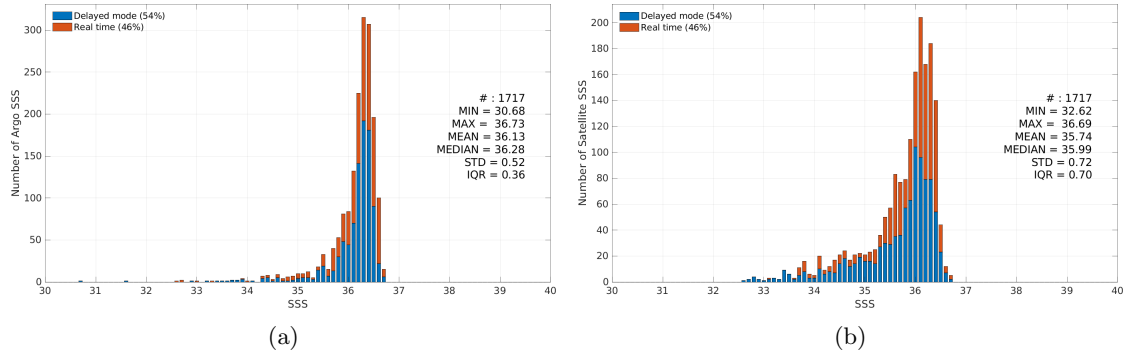
Figure 3: Histograms of SSS from Argo (a) and Aquarius SSS L4 OI v5 - Weekly (IPRC) (b) considering all match-up pairs per bins of 0.1 over the Gulf of Mexico Pi-MEP region and for the full satellite product period.
