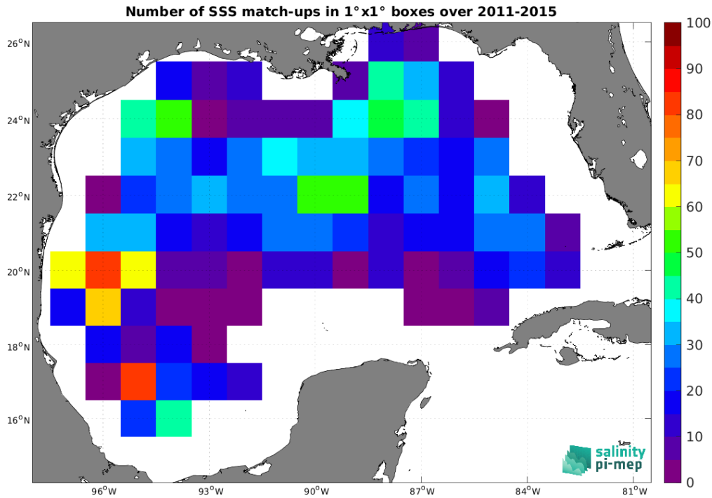
Figure 4: Number of SSS match-ups between Argo SSS and the Aquarius SSS L4 OI v5 - Weekly (IPRC) SSS product for the Gulf of Mexico Pi-MEP region over 1^\circ \times 1^\circ boxes and for the full satellite product period.
