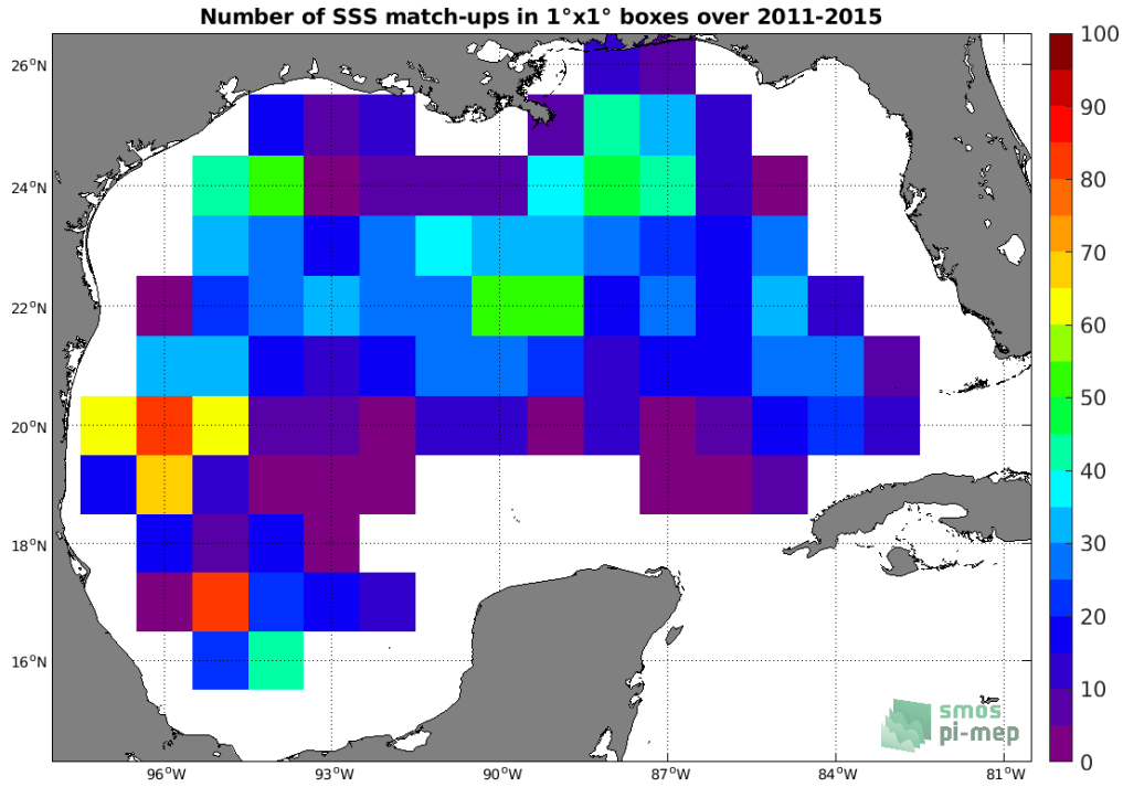
Figure 4: Number of SSS match-ups between Argo SSS and the Aquarius SSS L4 OI v5 - Weekly (IPRC) SSS product for the Gulf of Mexico Pi-MEP region over 1°×1° boxes and for the full satellite product period.
