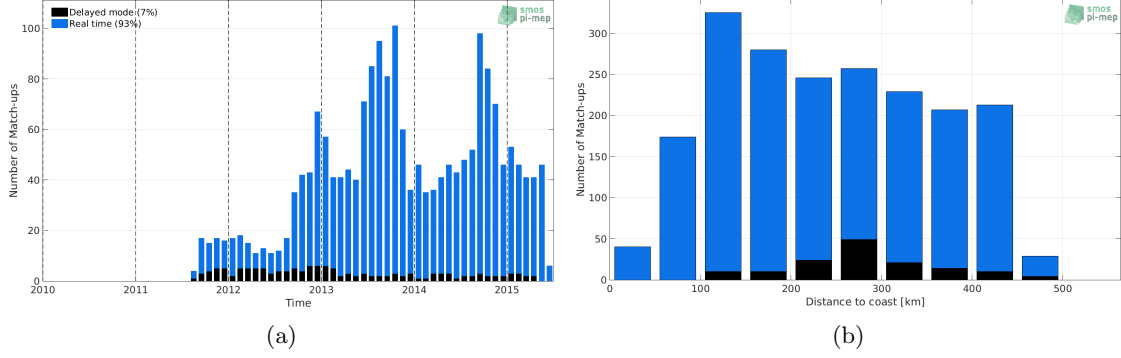
Figure 1: Number of match-ups between Argo and Aquarius-L4-IPRC-V5-WEEKLY SSS as a function of time (a) and as function of the distance to coast (b) over the Gulf of Mexico Pi-MEP region and for the full satellite product period.
