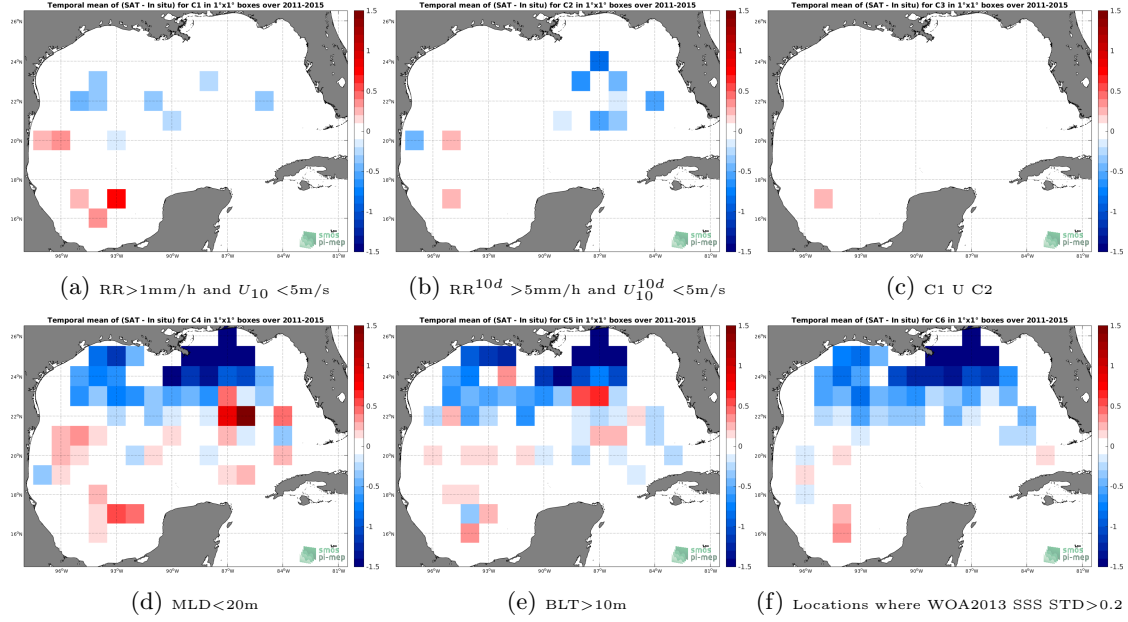
Figure 12: Temporal mean gridded over spatial boxes of size 1^\circ \times 1^\circ of \Delta\text{SSS} (Aquarius-L4-IPRC-V5-WEEKLY - Argo) for 6 different subdatasets corresponding to: RR > 1\text{mm/h} and U_{10} < 5\text{m/s} (a), RR^{10d} > 5\text{mm/h} and U_{10}^{10d} < 5\text{m/s} (b), C1 U C2 (c), MLD < 20\text{m} (d), BLT > 10\text{m} (e), Locations where WOA2013 SSS STD > 0.2 (f).
