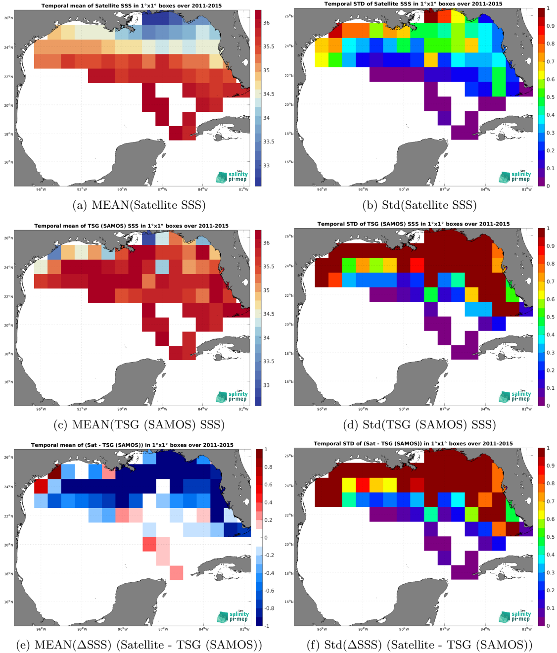
Figure 7: Temporal mean (left) and Std (right) of SSS from Aquarius SSS L4 OI v5 - Monthly (IPRC) (top), TSG (SAMOS) (middle), and of \Delta SSS (Satellite - TSG (SAMOS)). Only match-up pairs are used to generate these maps.
