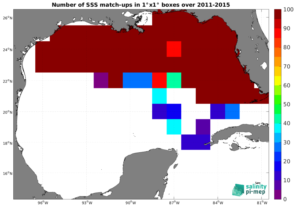
Figure 5: Number of SSS match-ups between TSG (SAMOS) SSS and the Aquarius SSS L4 OI v5 - Monthly (IPRC) SSS product for the Gulf of Mexico Pi-MEP region over 1^\circ \times 1^\circ boxes and for the full satellite product period.
