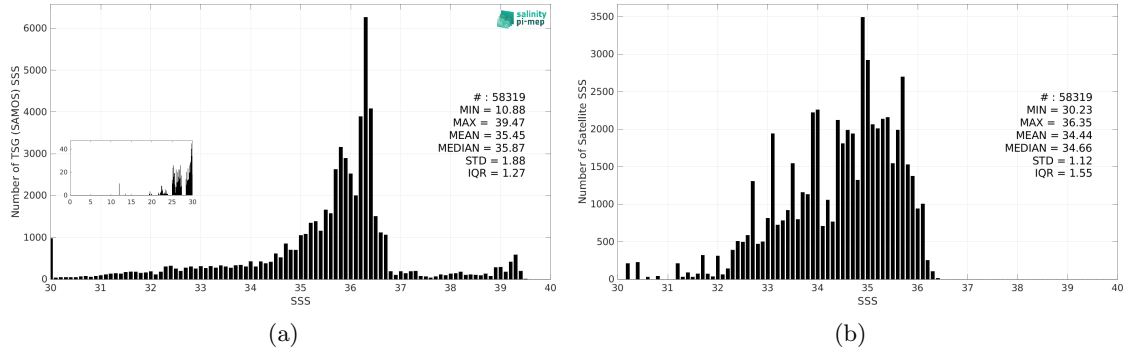
Figure 3: Histograms of SSS from TSG (SAMOS) (a) and Aquarius SSS L4 OI v5 - Monthly (IPRC) (b) considering all match-up pairs per bins of 0.1 over the Gulf of Mexico Pi-MEP region and for the full satellite product period.
