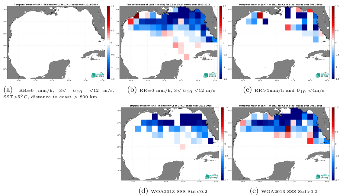
Figure 14: Temporal mean gridded over spatial boxes of size 1^\circ \times 1^\circ of \Delta SSS (Aquarius SSS L4 OI v5 - Monthly (IPRC) - TSG (SAMOS)) for 5 different subdatasets corresponding to:RR=0 mm/h, 3 < U_{10} < 12 m/s, SST > 5^\circ\text{C} , distance to coast > 800 km (a), RR=0 mm/h, 3 < U_{10} < 12 m/s (b), RR > 1 mm/h and U_{10} < 4 m/s (c), WOA2013 SSS Std < 0.2 (d), WOA2013 SSS Std > 0.2 (e).
