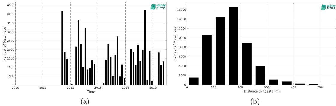
Figure 2: Number of match-ups between TSG (SAMOS) and Aquarius SSS L4 OI v5 - Monthly (IPRC) SSS as a function of time (a) and as function of the distance to coast (b) over the Gulf of Mexico Pi-MEP region and for the full satellite product period.
