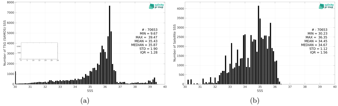
Figure 2: Histograms of SSS from TSG (SAMOS) (a) and Aquarius SSS L4 OI v5 - Monthly (IPRC) (b) considering all match-up pairs per bins of 0.1 over the Gulf of Mexico Pi-MEP region and for the full satellite product period.
