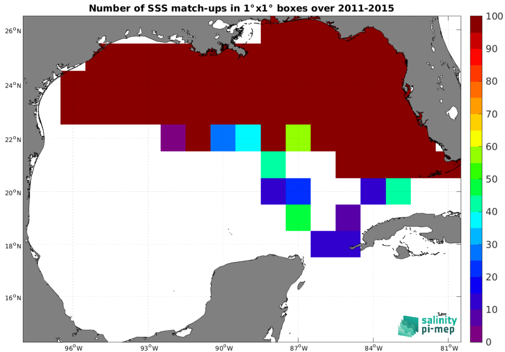
Figure 4: Number of SSS match-ups between TSG (SAMOS) SSS and the Aquarius SSS L4 OI v5 - Monthly (IPRC) SSS product for the Gulf of Mexico Pi-MEP region over 1^\circ \times 1^\circ boxes and for the full satellite product period.
