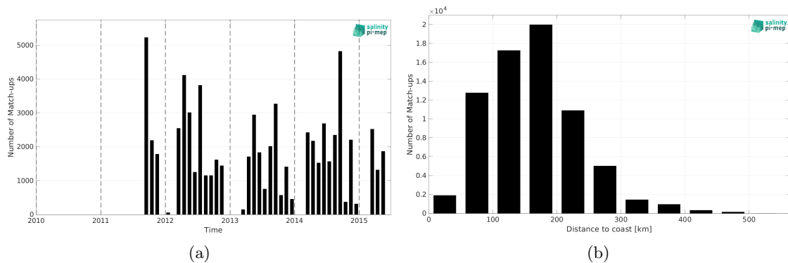
Figure 1: Number of match-ups between TSG (SAMOS) and Aquarius SSS L4 OI v5 - Monthly (IPRC) SSS as a function of time (a) and as function of the distance to coast (b) over the Gulf of Mexico Pi-MEP region and for the full satellite product period.
