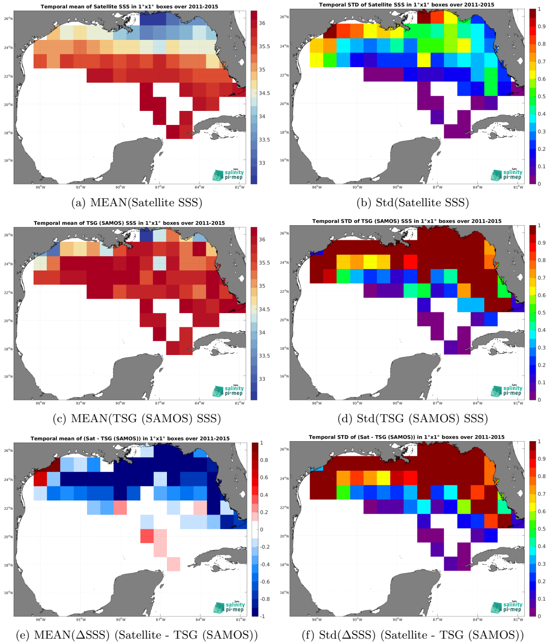
Figure 6: Temporal mean (left) and Std (right) of SSS from Aquarius SSS L4 OI v5 - Monthly (IPRC) (top), TSG (SAMOS) (middle), and of \Delta SSS (Satellite - TSG (SAMOS)). Only match-up pairs are used to generate these maps.
