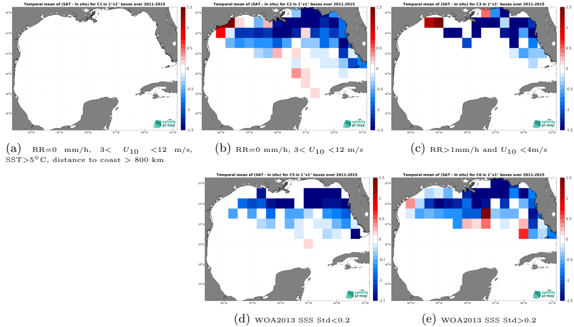
Figure 12: Temporal mean gridded over spatial boxes of size 1^{\circ}\times 1^{\circ} of \Delta\text{SSS} (Aquarius SSS L4 OI v5 - Monthly (IPRC) - TSG (SAMOS)) for 5 different subdatasets corresponding to:RR=0 mm/h, 3 < U_{10} < 12 m/s, SST >5^{\circ}\text{C} , distance to coast > 800 km (a), RR=0 mm/h, 3 < U_{10} < 12 m/s (b), RR >1 mm/h and U_{10} < 4 m/s (c), WOA2013 SSS Std <0.2 (d), WOA2013 SSS Std >0.2 (e).
