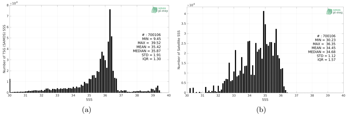
Figure 2: Histograms of SSS from TSG (SAMOS) (a) and Aquarius SSS L4 OI v5 - Monthly (IPRC) (b) considering all match-up pairs per bins of 0.1 over the Gulf of Mexico Pi-MEP region and for the full satellite product period.
