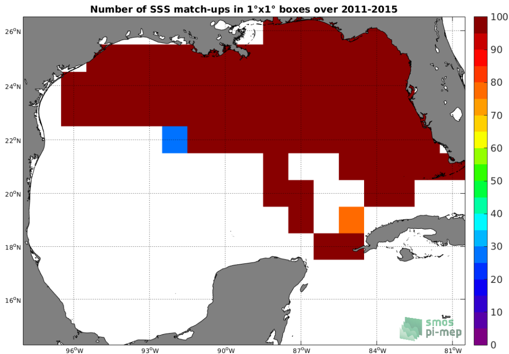
Figure 4: Number of SSS match-ups between TSG-SAMOS SSS and the Aquarius-L4-IPRC-V5-MONTHLY SSS product for the Gulf of Mexico Pi-MEP region over 1°x1° boxes and for the full satellite product period.
