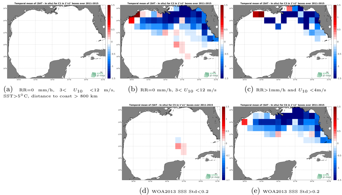
Figure 12: Temporal mean gridded over spatial boxes of size 1^{\circ}\times 1^{\circ} of \Delta\text{SSS} (Aquarius-L4-IPRC-V5-MONTHLY - TSG-SAMOS) for 5 different subdatasets corresponding to:RR=0 mm/h, 3 < U_{10} < 12 m/s, SST >5^{\circ}\text{C} , distance to coast > 800 km (a), RR=0 mm/h, 3 < U_{10} < 12 m/s (b), RR >1 mm/h and U_{10} < 4 m/s (c), WOA2013 SSS Std <0.2 (d), WOA2013 SSS Std >0.2 (e).
