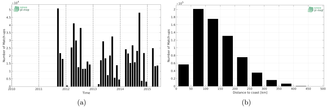
Figure 1: Number of match-ups between TSG-SAMOS and Aquarius-L4-IPRC-V5-MONTHLY SSS as a function of time (a) and as function of the distance to coast (b) over the Gulf of Mexico Pi-MEP region and for the full satellite product period.
