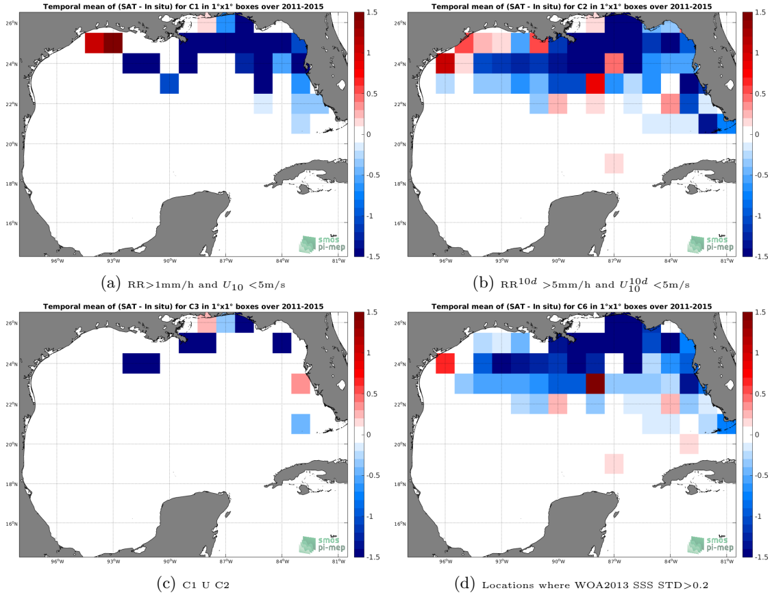
Figure 12: Temporal mean gridded over spatial boxes of size 1^\circ \times 1^\circ of \Delta SSS (Aquarius-L4-IPRC-V5-MONTHLY - TSG-SAMOS) for 4 different subdatasets corresponding to: RR > 1\text{mm/h} and U_{10} < 5\text{m/s} (a), RR^{10d} > 5\text{mm/h} and U_{10}^{10d} < 5\text{m/s} (b), C1 U C2 (c), Locations where WOA2013 SSS STD > 0.2 (d).
