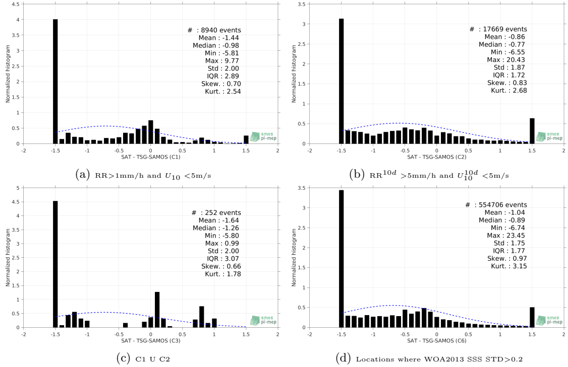
Figure 13: Normalized histogram of \Delta SSS (Aquarius-L4-IPRC-V5-MONTHLY - TSG-SAMOS) for 6 different subdatasets corresponding to: RR > 1mm/h and U_{10} < 5 m/s (a), RR^{10d} > 5 mm/h and U_{10}^{10d} < 5 m/s (b), C1 U C2 (c), Locations where WOA2013 SSS STD > 0.2 (d).
