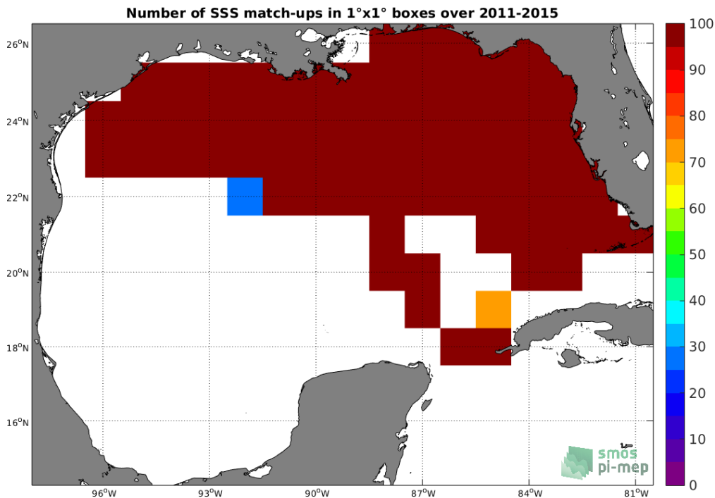
Figure 4: Number of SSS match-ups between TSG-SAMOS SSS and the Aquarius-L4-IPRC-V5-MONTHLY SSS product for the Gulf of Mexico Pi-MEP region over 1^{\circ} \times 1^{\circ} boxes and for the full satellite product period.
