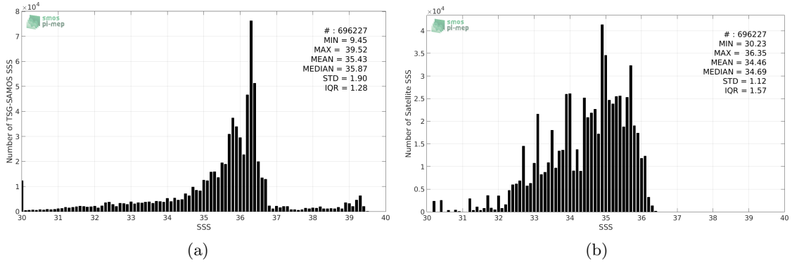
Figure 2: Histograms of SSS from TSG-SAMOS (a) and Aquarius-L4-IPRC-V5-MONTHLY (b) considering all match-up pairs per bins of 0.1 over the Gulf of Mexico Pi-MEP region and for the full satellite product period.
