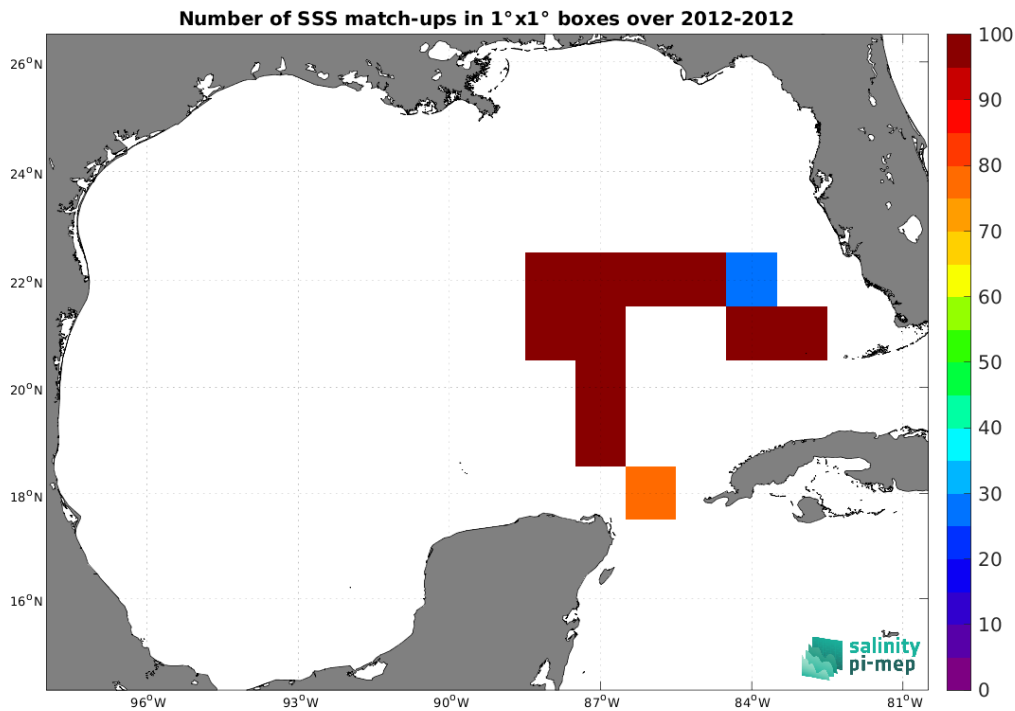
Figure 5: Number of SSS match-ups between TSG (GOSUD-Sailing-ship) SSS and the Aquarius SSS L4 OI v5 - Monthly (IPRC) SSS product for the Gulf of Mexico Pi-MEP region over 1^\circ \times 1^\circ boxes and for the full satellite product period.
