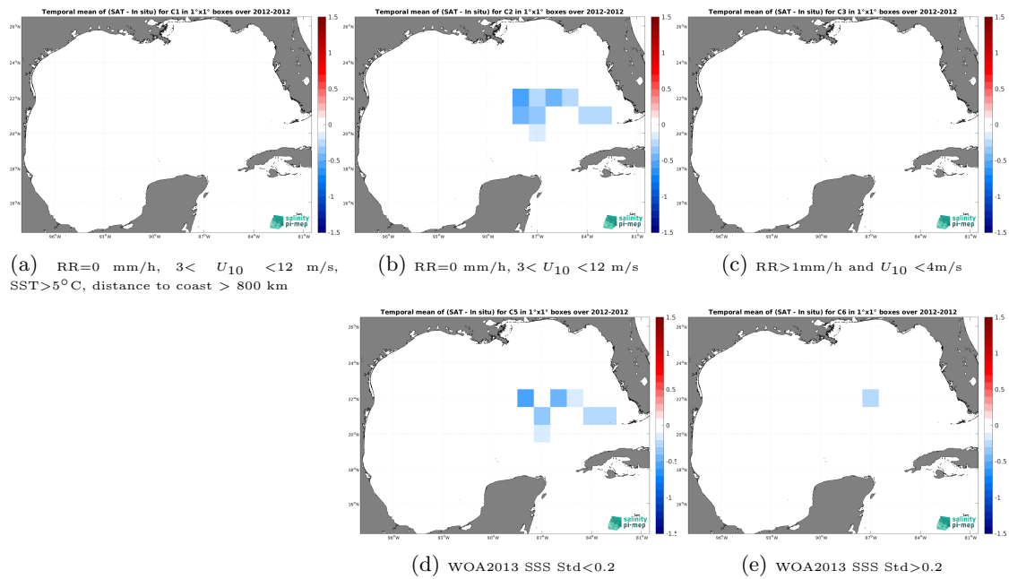
Figure 14: Temporal mean gridded over spatial boxes of size 1^\circ \times 1^\circ of \Delta SSS (Aquarius SSS L4 OI v5 - Monthly (IPRC) - TSG (GOSUD-Sailing-ship)) for 5 different subdatasets corresponding to:RR=0 mm/h, 3 < U_{10} < 12 m/s, SST >5^\circ C, distance to coast > 800 km (a), RR=0 mm/h, 3 < U_{10} < 12 m/s (b), RR >1 mm/h and U_{10} < 4 m/s (c), WOA2013 SSS Std <0.2 (d), WOA2013 SSS Std >0.2 (e).
