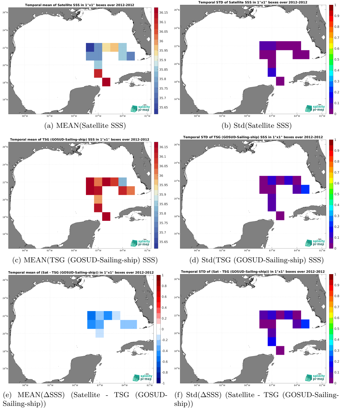
Figure 7: Temporal mean (left) and Std (right) of SSS from Aquarius SSS L4 OI v5 - Monthly (IPRC) (top), TSG (GOSUD-Sailing-ship) (middle), and of \Delta SSS (Satellite - TSG (GOSUD-Sailing-ship)). Only match-up pairs are used to generate these maps.
