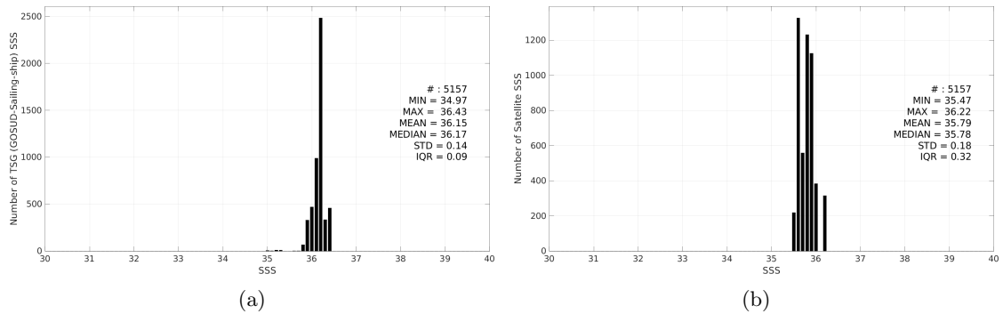
Figure 3: Histograms of SSS from TSG (GOSUD-Sailing-ship) (a) and Aquarius SSS L4 OI v5 - Monthly (IPRC) (b) considering all match-up pairs per bins of 0.1 over the Gulf of Mexico Pi-MEP region and for the full satellite product period.
