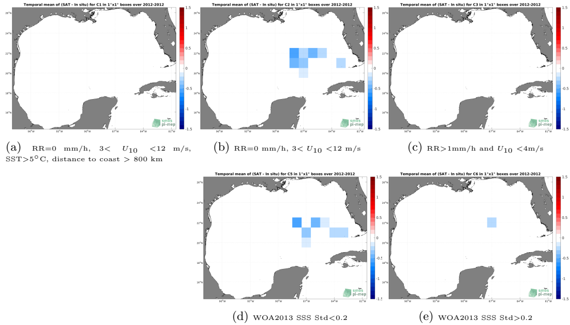
Figure 12: Temporal mean gridded over spatial boxes of size 1^\circ \times 1^\circ of \Delta SSS (Aquarius SSS L4 OI v5 - Monthly (IPRC) - TSG (GOSUD-Sailing-ship)) for 5 different subdatasets corresponding to:RR=0 mm/h, 3 < U_{10} < 12 m/s, SST >5^\circ\text{C} , distance to coast > 800 km (a), RR=0 mm/h, 3 < U_{10} < 12 m/s (b), RR >1 mm/h and U_{10} < 4 m/s (c), WOA2013 SSS Std <0.2 (d), WOA2013 SSS Std >0.2 (e).
