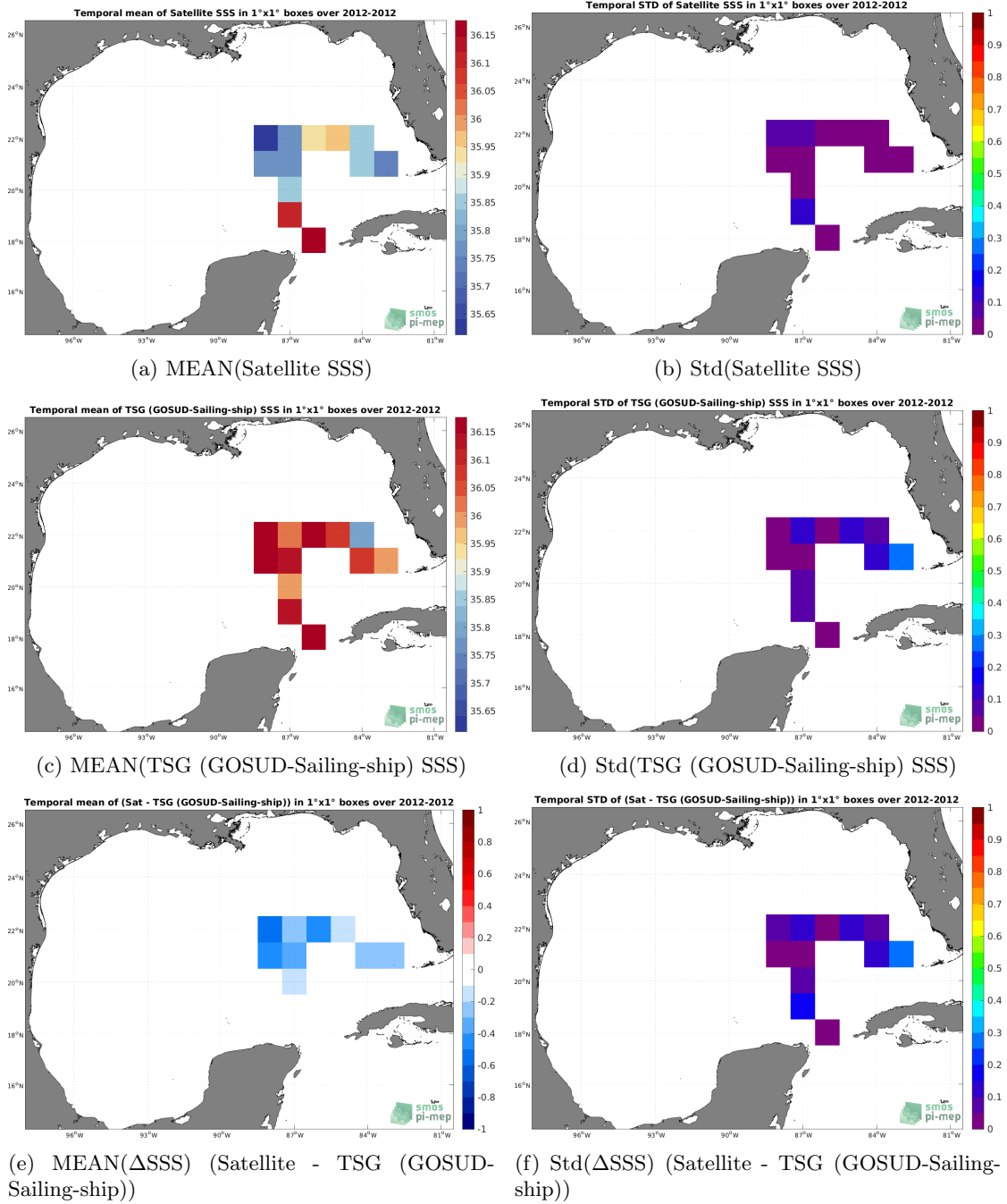
Figure 6: Temporal mean (left) and Std (right) of SSS from Aquarius SSS L4 OI v5 - Monthly (IPRC) (top), TSG (GOSUD-Sailing-ship) (middle), and of \Delta SSS (Satellite - TSG (GOSUD-Sailing-ship)). Only match-up pairs are used to generate these maps.
