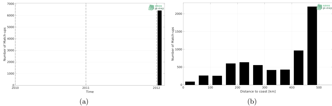
Figure 1: Number of match-ups between TSG (GOSUD-Sailing-ship) and Aquarius SSS L4 OI v5 - Monthly (IPRC) SSS as a function of time (a) and as function of the distance to coast (b) over the Gulf of Mexico Pi-MEP region and for the full satellite product period.
