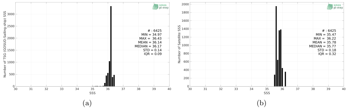
Figure 2: Histograms of SSS from TSG (GOSUD-Sailing-ship) (a) and Aquarius SSS L4 OI v5 - Monthly (IPRC) (b) considering all match-up pairs per bins of 0.1 over the Gulf of Mexico Pi-MEP region and for the full satellite product period.
