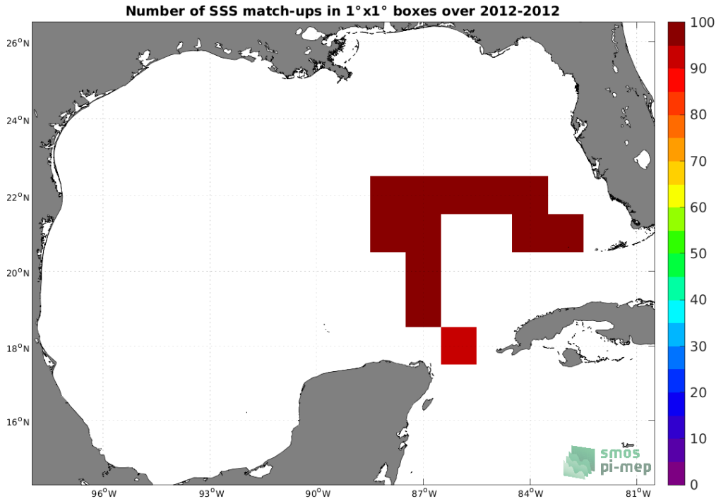
Figure 4: Number of SSS match-ups between TSG (GOSUD-Sailing-ship) SSS and the Aquarius SSS L4 OI v5 - Monthly (IPRC) SSS product for the Gulf of Mexico Pi-MEP region over 1^\circ \times 1^\circ boxes and for the full satellite product period.
