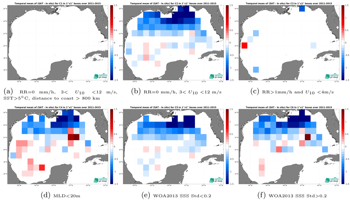
Figure 14: Temporal mean gridded over spatial boxes of size 1^\circ \times 1^\circ of \Delta SSS (Aquarius SSS L4 OI v5 - Monthly (IPRC) - Argo) for 6 different subdatasets corresponding to:RR=0 mm/h, 3 < U_{10} < 12 m/s, SST > 5^\circ\text{C} , distance to coast > 800 km (a), RR=0 mm/h, 3 < U_{10} < 12 m/s (b), RR > 1 mm/h and U_{10} < 4 m/s (c),MLD < 20 m (d),WOA2013 SSS Std < 0.2 (e),WOA2013 SSS Std > 0.2 (f).
