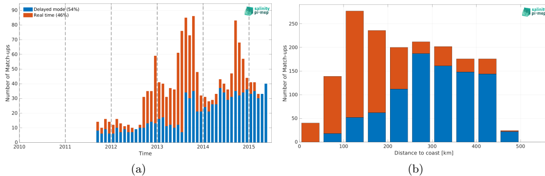
Figure 2: Number of match-ups between Argo and Aquarius SSS L4 OI v5 - Monthly (IPRC) SSS as a function of time (a) and as function of the distance to coast (b) over the Gulf of Mexico Pi-MEP region and for the full satellite product period.
