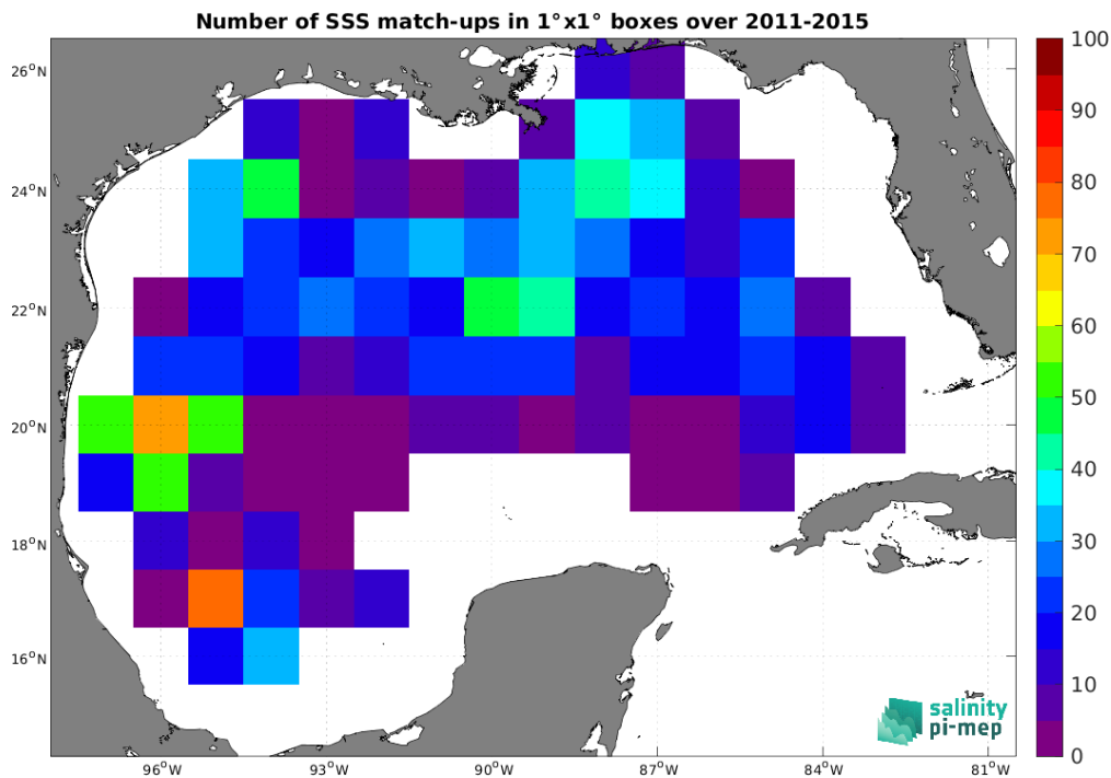
Figure 5: Number of SSS match-ups between Argo SSS and the Aquarius SSS L4 OI v5 - Monthly (IPRC) SSS product for the Gulf of Mexico Pi-MEP region over 1^{\circ} \times 1^{\circ} boxes and for the full satellite product period.
