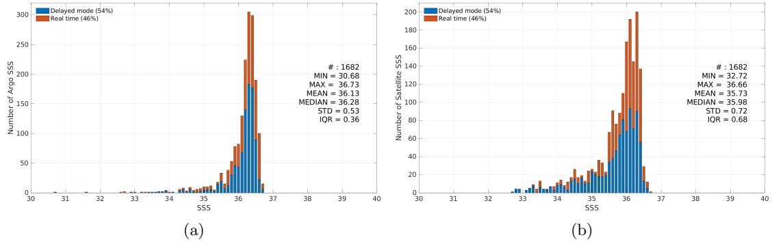
Figure 3: Histograms of SSS from Argo (a) and Aquarius SSS L4 OI v5 - Monthly (IPRC) (b) considering all match-up pairs per bins of 0.1 over the Gulf of Mexico Pi-MEP region and for the full satellite product period.
