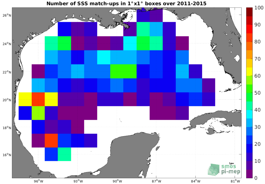
Figure 4: Number of SSS match-ups between Argo SSS and the Aquarius SSS L4 OI v5 - Monthly (IPRC) SSS product for the Gulf of Mexico Pi-MEP region over 1°x1° boxes and for the full satellite product period.
