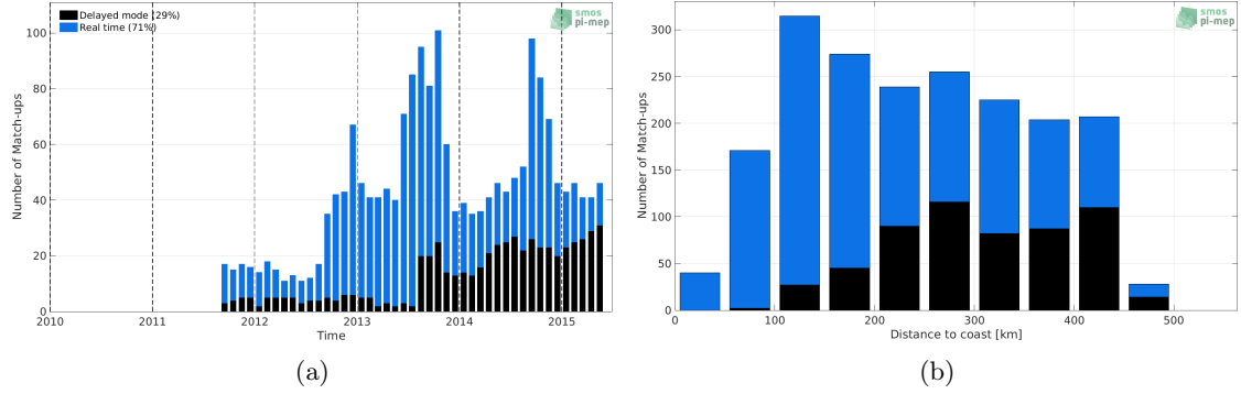
Figure 1: Number of match-ups between Argo and Aquarius SSS L4 OI v5 - Monthly (IPRC) SSS as a function of time (a) and as function of the distance to coast (b) over the Gulf of Mexico Pi-MEP region and for the full satellite product period.
