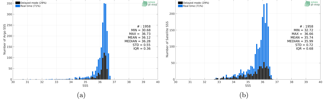
Figure 2: Histograms of SSS from Argo (a) and Aquarius SSS L4 OI v5 - Monthly (IPRC) (b) considering all match-up pairs per bins of 0.1 over the Gulf of Mexico Pi-MEP region and for the full satellite product period.
