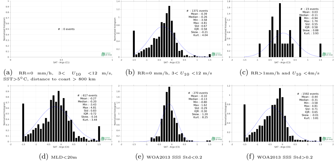
Figure 13: Normalized histogram of \Delta SSS (Aquarius SSS L4 OI v5 - Monthly (IPRC) - Argo) for 6 different subdatasets corresponding to: RR=0 mm/h, 3 < U_{10} < 12 m/s, SST > 5^\circ C , distance to coast > 800 km (a), RR=0 mm/h, 3 < U_{10} < 12 m/s (b), RR > 1 mm/h and U_{10} < 4 m/s (c), MLD < 20 m (d), WOA2013 SSS Std < 0.2 (e), WOA2013 SSS Std > 0.2 (f).
