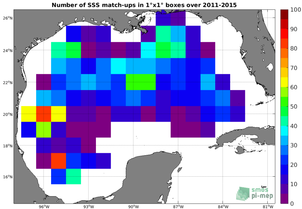
Figure 4: Number of SSS match-ups between Argo SSS and the Aquarius SSS L4 OI v5 - Monthly (IPRC) SSS product for the Gulf of Mexico Pi-MEP region over 1^\circ \times 1^\circ boxes and for the full satellite product period.
