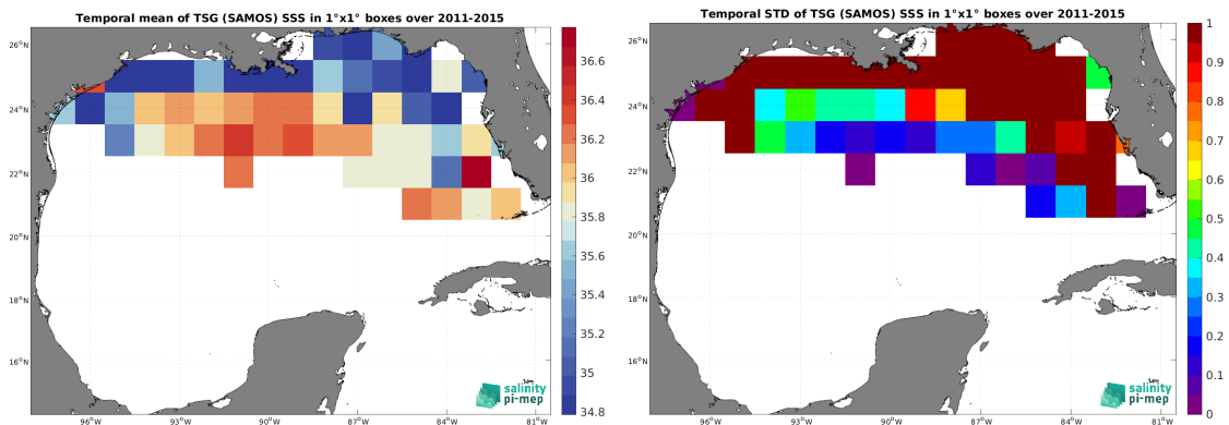
(c) MEAN(TSG (SAMOS) SSS)
