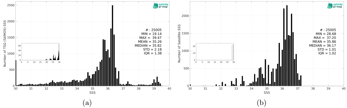
Figure 3: Histograms of SSS from TSG (SAMOS) (a) and Aquarius SSS L3 OR v5 - 7-Day running (NASA-GSFC) (b) considering all match-up pairs per bins of 0.1 over the Gulf of Mexico Pi-MEP region and for the full satellite product period.
