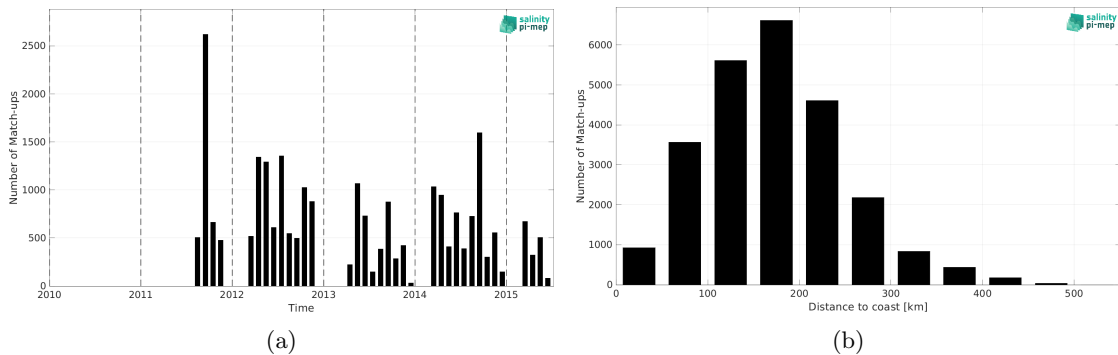
Figure 2: Number of match-ups between TSG (SAMOS) and Aquarius SSS L3 OR v5 - 7-Day running (NASA-GSFC) SSS as a function of time (a) and as function of the distance to coast (b) over the Gulf of Mexico Pi-MEP region and for the full satellite product period.
