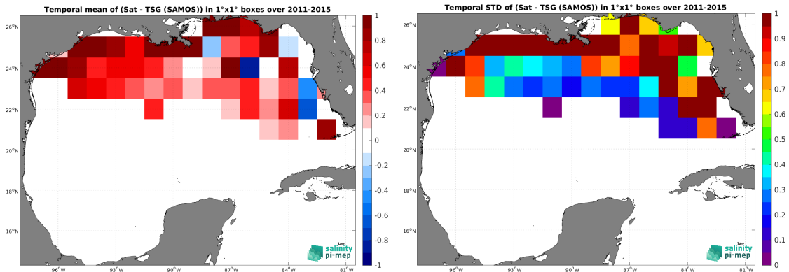
(e) MEAN( \Delta SSS) (Satellite - TSG (SAMOS))
