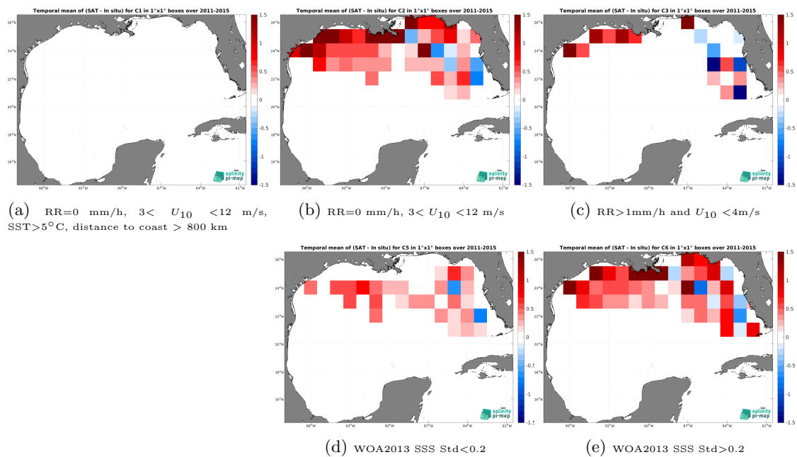
Figure 14: Temporal mean gridded over spatial boxes of size 1^\circ \times 1^\circ of \Delta SSS (Aquarius SSS L3 OR v5 - 7-Day running (NASA-GSFC) - TSG (SAMOS)) for 5 different subdatasets corresponding to:RR=0 mm/h, 3 < U_{10} < 12 m/s, SST >5^\circ C, distance to coast > 800 km (a), RR=0 mm/h, 3 < U_{10} < 12 m/s (b), RR >1 mm/h and U_{10} < 4 m/s (c), WOA2013 SSS Std <0.2 (d), WOA2013 SSS Std >0.2 (e).
