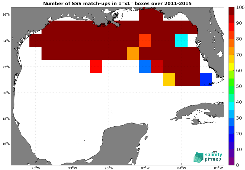
Figure 5: Number of SSS match-ups between TSG (SAMOS) SSS and the Aquarius SSS L3 OR v5 - 7-Day running (NASA-GSFC) SSS product for the Gulf of Mexico Pi-MEP region over 1^\circ \times 1^\circ boxes and for the full satellite product period.
