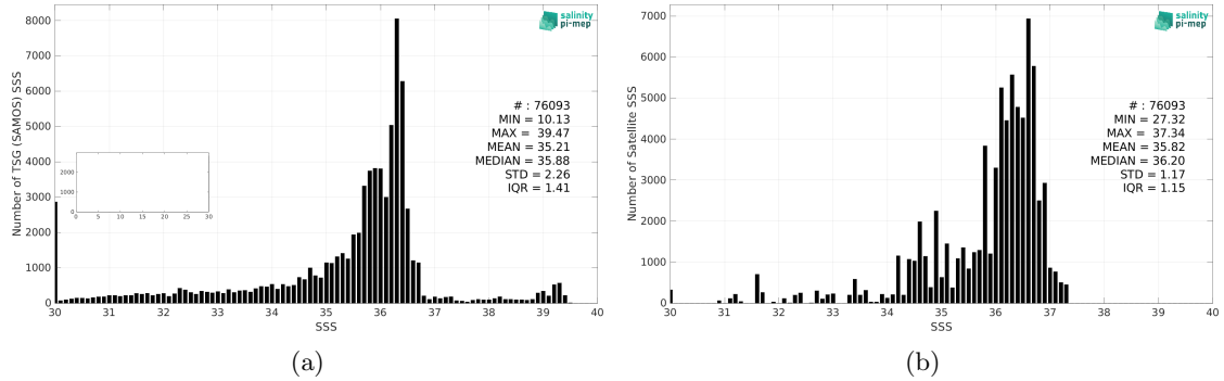
Figure 2: Histograms of SSS from TSG (SAMOS) (a) and Aquarius SSS L3 OR v5 - 7-Day running (NASA-GSFC) (b) considering all match-up pairs per bins of 0.1 over the Gulf of Mexico Pi-MEP region and for the full satellite product period.
