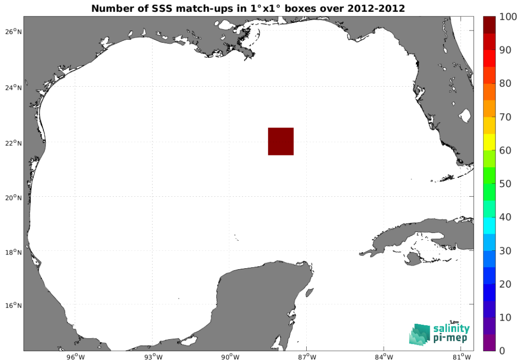
Figure 5: Number of SSS match-ups between TSG (GOSUD-Sailing-ship) SSS and the Aquarius SSS L3 OR v5 - 7-Day running (NASA-GSFC) SSS product for the Gulf of Mexico Pi-MEP region over 1^\circ \times 1^\circ boxes and for the full satellite product period.
