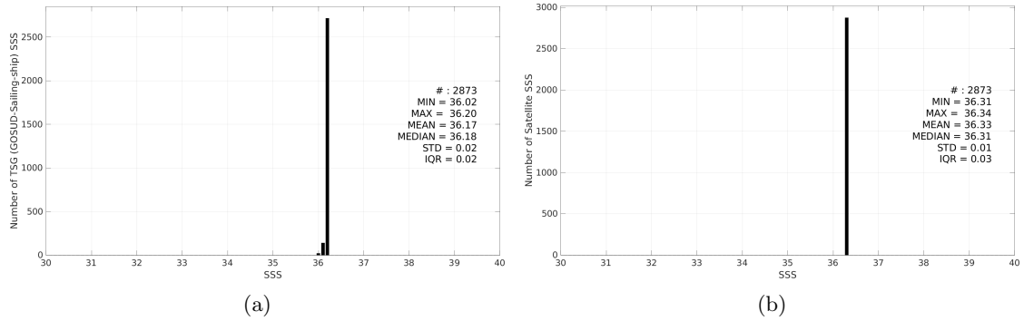
Figure 3: Histograms of SSS from TSG (GOSUD-Sailing-ship) (a) and Aquarius SSS L3 OR v5 - 7-Day running (NASA-GSFC) (b) considering all match-up pairs per bins of 0.1 over the Gulf of Mexico Pi-MEP region and for the full satellite product period.
