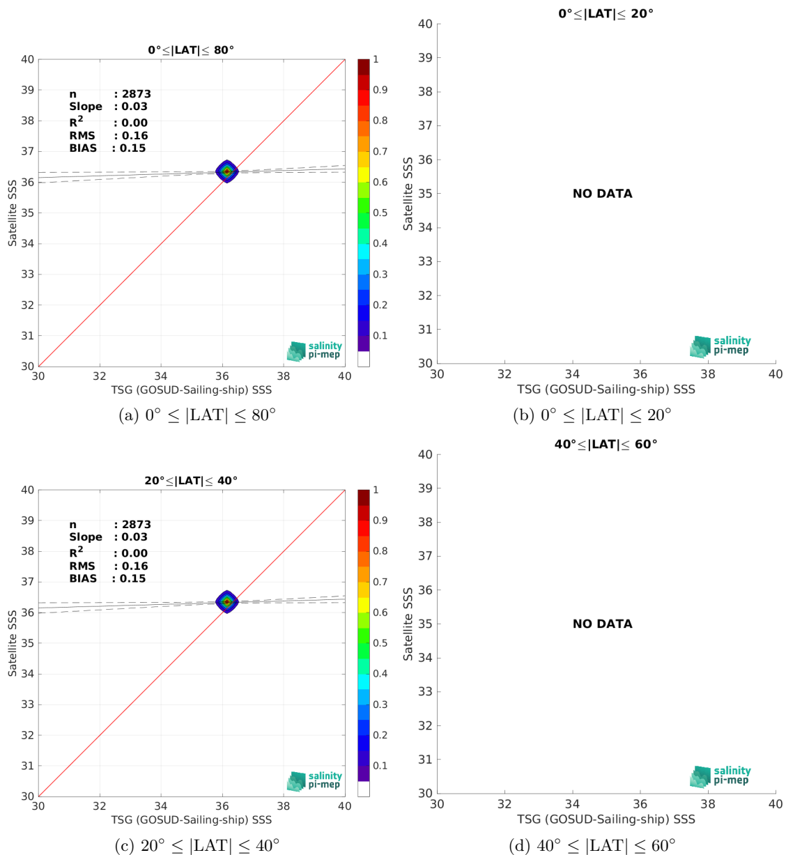
Figure 10: Contour maps of the concentration of Aquarius SSS L3 OR v5 - 7-Day running (NASA-GSFC) SSS (y-axis) versus TSG (GOSUD-Sailing-ship) SSS (x-axis) at match-up pairs for different latitude bands. For each plot, the red line shows x=y . The black thin and dashed lines indicate a linear fit through the data cloud and the \pm 95\% confidence levels, respectively. The number match-up pairs n , the slope and R^2 coefficient of the linear fit, the root mean square (RMS) and the mean bias between satellite and in situ data are indicated for each latitude band in each plots.
