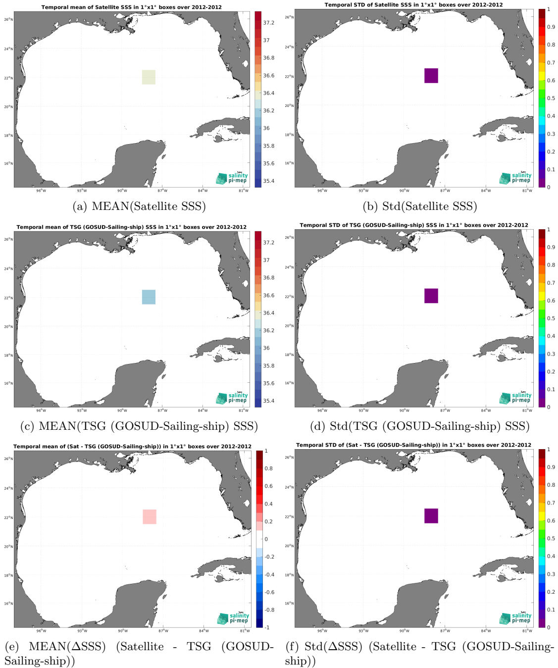
Figure 7: Temporal mean (left) and Std (right) of SSS from Aquarius SSS L3 OR v5 - 7-Day running (NASA-GSFC) (top), TSG (GOSUD-Sailing-ship) (middle), and of \Delta SSS (Satellite - TSG (GOSUD-Sailing-ship)). Only match-up pairs are used to generate these maps.
