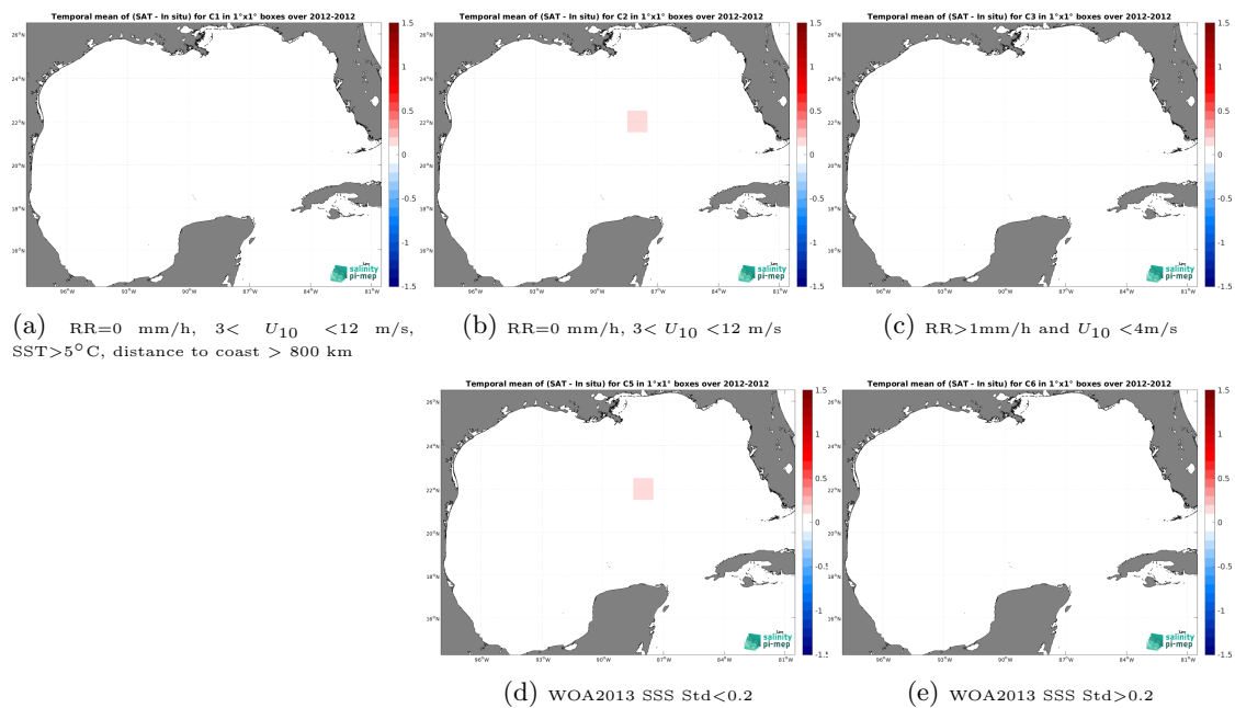
Figure 14: Temporal mean gridded over spatial boxes of size 1^\circ \times 1^\circ of \Delta\text{SSS} (Aquarius SSS L3 OR v5 - 7-Day running (NASA-GSFC) - TSG (GOSUD-Sailing-ship)) for 5 different subdatasets corresponding to:RR=0 mm/h, 3 < U_{10} < 12 m/s, SST >5^\circ\text{C} , distance to coast > 800 km (a), RR=0 mm/h, 3 < U_{10} < 12 m/s (b), RR >1 mm/h and U_{10} < 4 m/s (c), WOA2013 SSS Std <0.2 (d), WOA2013 SSS Std >0.2 (e).
