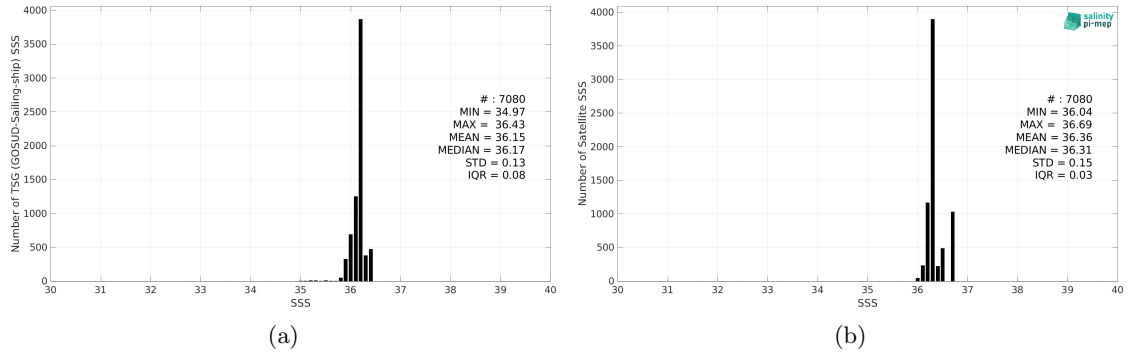
Figure 2: Histograms of SSS from TSG (GOSUD-Sailing-ship) (a) and Aquarius SSS L3 OR v5 - 7-Day running (NASA-GSFC) (b) considering all match-up pairs per bins of 0.1 over the Gulf of Mexico Pi-MEP region and for the full satellite product period.
