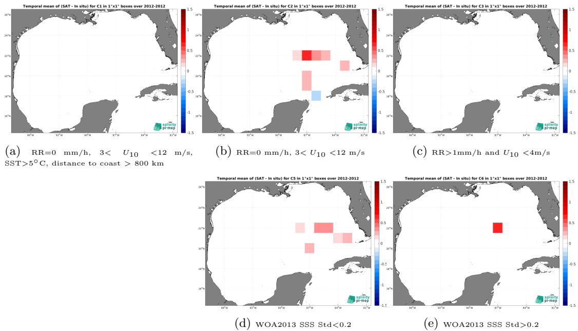
Figure 12: Temporal mean gridded over spatial boxes of size 1^\circ \times 1^\circ of \Delta SSS (Aquarius SSS L3 OR v5 - 7-Day running (NASA-GSFC) - TSG (GOSUD-Sailing-ship)) for 5 different subdatasets corresponding to:RR=0 mm/h, 3 < U_{10} < 12 m/s, SST >5^\circ\text{C} , distance to coast > 800 km (a), RR=0 mm/h, 3 < U_{10} < 12 m/s (b), RR >1 mm/h and U_{10} < 4 m/s (c), WOA2013 SSS Std <0.2 (d), WOA2013 SSS Std >0.2 (e).
