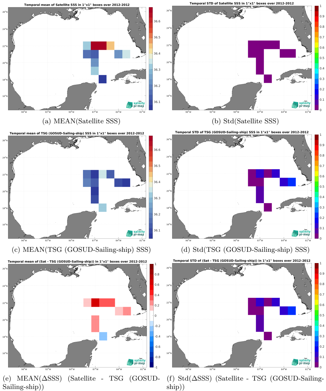
Figure 6: Temporal mean (left) and Std (right) of SSS from Aquarius SSS L3 OR v5 - 7-Day running (NASA-GSFC) (top), TSG (GOSUD-Sailing-ship) (middle), and of \Delta SSS (Satellite - TSG (GOSUD-Sailing-ship)). Only match-up pairs are used to generate these maps.
