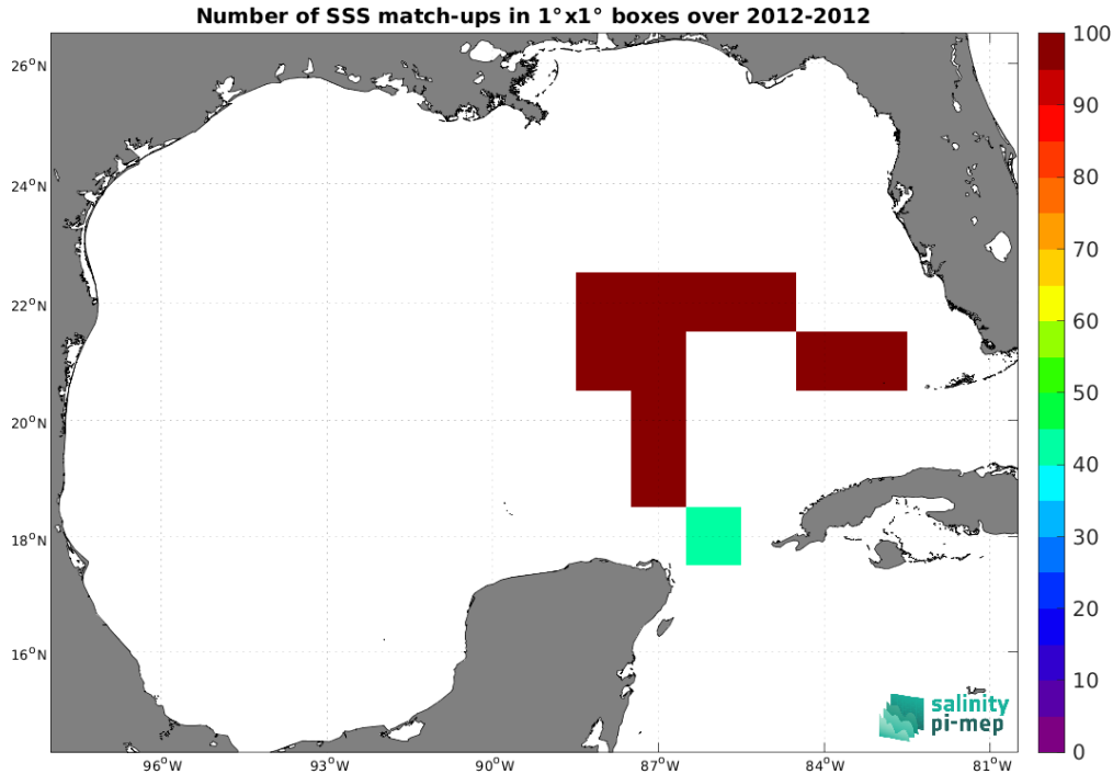
Figure 4: Number of SSS match-ups between TSG (GOSUD-Sailing-ship) SSS and the Aquarius SSS L3 OR v5 - 7-Day running (NASA-GSFC) SSS product for the Gulf of Mexico Pi-MEP region over 1^\circ \times 1^\circ boxes and for the full satellite product period.
