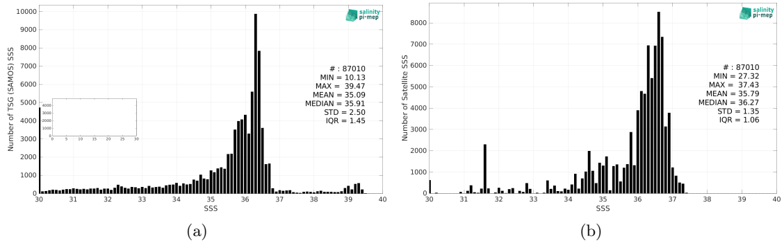
Figure 2: Histograms of SSS from TSG (SAMOS) (a) and Aquarius SSS L3 OR v5 - 7-Day running - Rain mask (NASA-GSFC) (b) considering all match-up pairs per bins of 0.1 over the Gulf of Mexico Pi-MEP region and for the full satellite product period.
