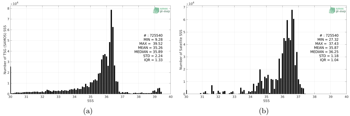
Figure 2: Histograms of SSS from TSG (SAMOS) (a) and Aquarius SSS L3 OR v5 - 7-Day running - Rain mask (NASA-GSFC) (b) considering all match-up pairs per bins of 0.1 over the Gulf of Mexico Pi-MEP region and for the full satellite product period.
