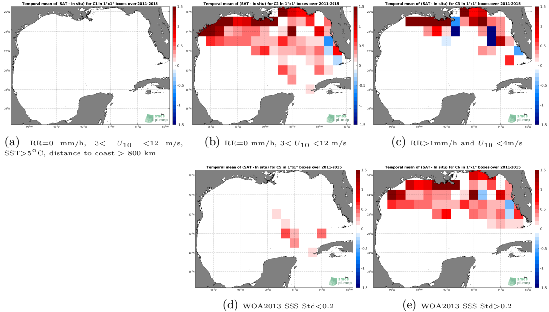
Figure 12: Temporal mean gridded over spatial boxes of size 1^{\circ}\times 1^{\circ} of \Delta\text{SSS} (Aquarius SSS L3 OR v5 - 7-Day running - Rain mask (NASA-GSFC) - TSG (SAMOS)) for 5 different subdatasets corresponding to:RR=0 mm/h, 3 < U_{10} < 12 m/s, SST >5^{\circ}\text{C} , distance to coast > 800 km (a), RR=0 mm/h, 3 < U_{10} < 12 m/s (b), RR >1 mm/h and U_{10} < 4 m/s (c), WOA2013 SSS Std <0.2 (d), WOA2013 SSS Std >0.2 (e).
