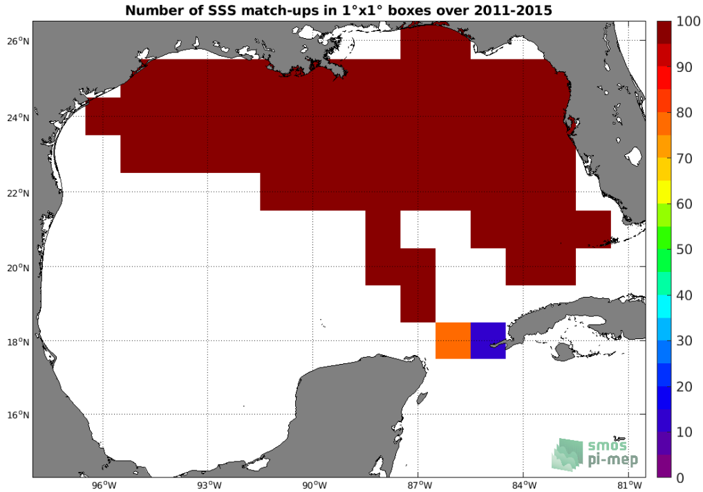
Figure 4: Number of SSS match-ups between TSG (SAMOS) SSS and the Aquarius SSS L3 OR v5 - 7-Day running - Rain mask (NASA-GSFC) SSS product for the Gulf of Mexico Pi-MEP region over 1^\circ \times 1^\circ boxes and for the full satellite product period.
