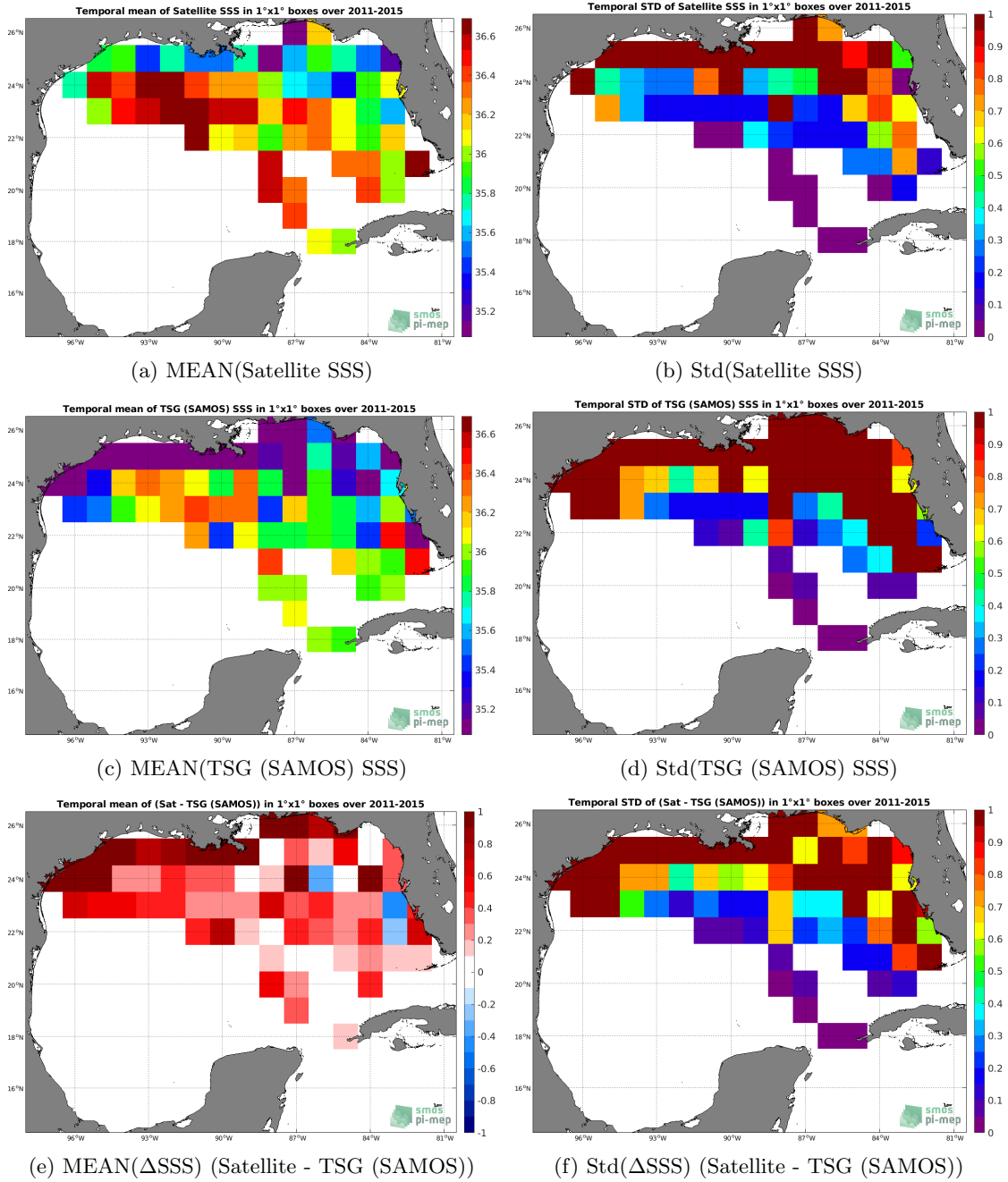
Figure 6: Temporal mean (left) and Std (right) of SSS from Aquarius SSS L3 OR v5 - 7-Day running - Rain mask (NASA-GSFC) (top), TSG (SAMOS) (middle), and of \Delta SSS (Satellite - TSG (SAMOS)). Only match-up pairs are used to generate these maps.
