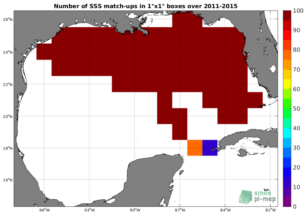
Figure 4: Number of SSS match-ups between TSG-SAMOS SSS and the Aquarius-L3-OR-V5-7DAY-RUNNING-RAIN-MASK-1DEG SSS product for the Gulf of Mexico Pi-MEP region over 1^\circ \times 1^\circ boxes and for the full satellite product period.
