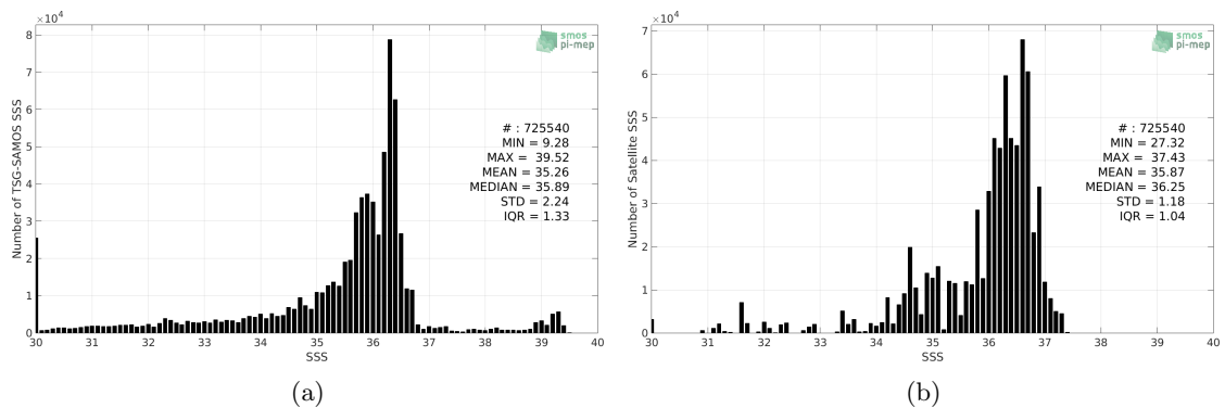
Figure 2: Histograms of SSS from TSG-SAMOS (a) and Aquarius-L3-OR-V5-7DAY-RUNNING-RAIN-MASK-1DEG (b) considering all match-up pairs per bins of 0.1 over the Gulf of Mexico Pi-MEP region and for the full satellite product period.
