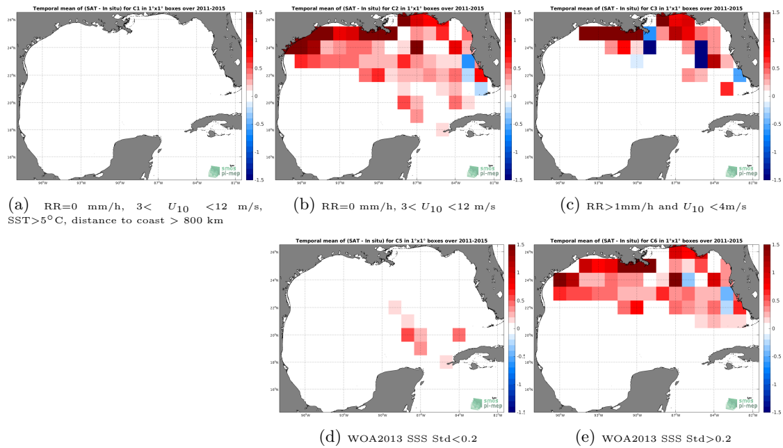
Figure 12: Temporal mean gridded over spatial boxes of size 1^\circ \times 1^\circ of \Delta SSS (Aquarius-L3-OR-V5-7DAY-RUNNING-RAIN-MASK-1DEG - TSG-SAMOS) for 5 different subdatasets corresponding to:RR=0 mm/h, 3 < U_{10} < 12 m/s, SST >5^\circ C, distance to coast > 800 km (a), RR=0 mm/h, 3 < U_{10} < 12 m/s (b), RR >1 mm/h and U_{10} < 4 m/s (c), WOA2013 SSS Std <0.2 (d), WOA2013 SSS Std >0.2 (e).
