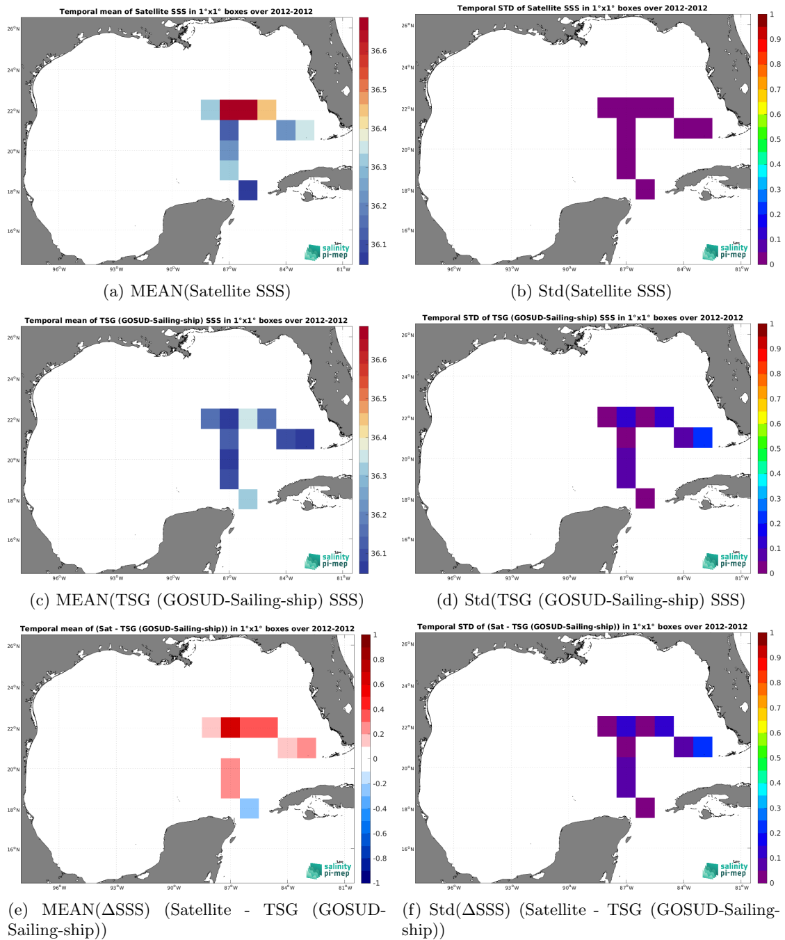
Figure 7: Temporal mean (left) and Std (right) of SSS from Aquarius SSS L3 OR v5 - 7-Day running - Rain mask (NASA-GSFC) (top), TSG (GOSUD-Sailing-ship) (middle), and of \Delta SSS (Satellite - TSG (GOSUD-Sailing-ship)). Only match-up pairs are used to generate these maps.
