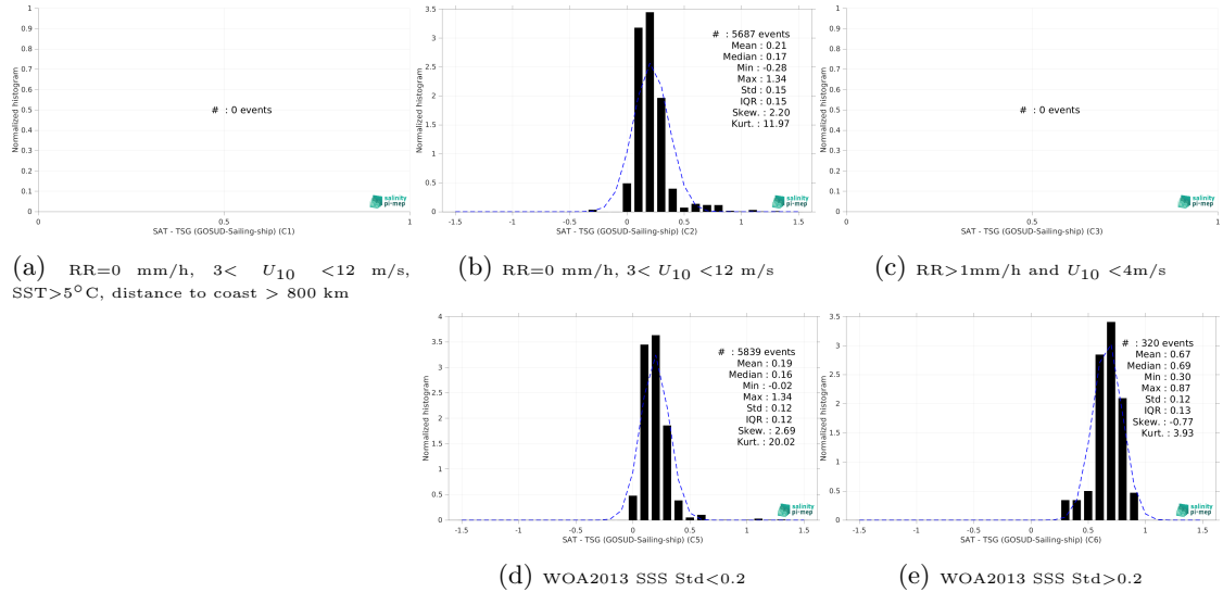
Figure 15: Normalized histogram of \Delta SSS (Aquarius SSS L3 OR v5 - 7-Day running - Rain mask (NASA-GSFC) - TSG (GOSUD-Sailing-ship)) for 5 different subdatasets corresponding to: RR=0 mm/h, 3 < U_{10} < 12 m/s, SST > 5°C, distance to coast > 800 km (a), RR=0 mm/h, 3 < U_{10} < 12 m/s (b), RR > 1mm/h and U_{10} < 4 m/s (c), WOA2013 SSS Std < 0.2 (d), WOA2013 SSS Std > 0.2 (e).
