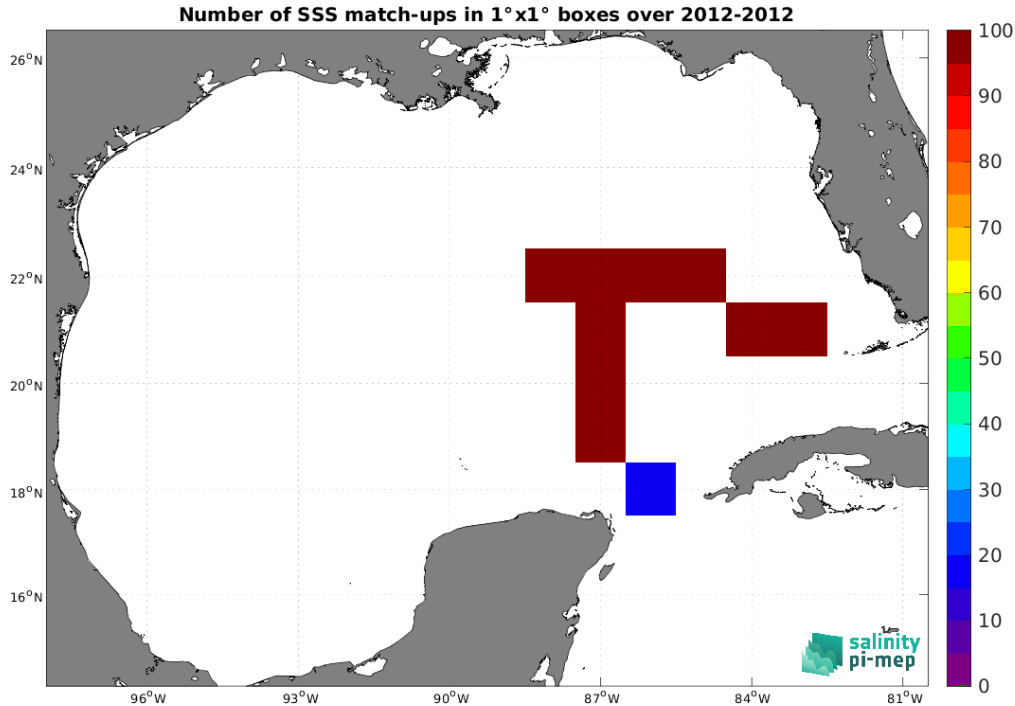
Figure 5: Number of SSS match-ups between TSG (GOSUD-Sailing-ship) SSS and the Aquarius SSS L3 OR v5 - 7-Day running - Rain mask (NASA-GSFC) SSS product for the Gulf of Mexico Pi-MEP region over 1^\circ \times 1^\circ boxes and for the full satellite product period.
