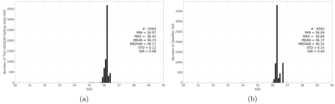
Figure 3: Histograms of SSS from TSG (GOSUD-Sailing-ship) (a) and Aquarius SSS L3 OR v5 - 7-Day running - Rain mask (NASA-GSFC) (b) considering all match-up pairs per bins of 0.1 over the Gulf of Mexico Pi-MEP region and for the full satellite product period.
