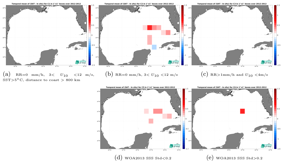
Figure 14: Temporal mean gridded over spatial boxes of size 1^\circ \times 1^\circ of \Delta SSS (Aquarius SSS L3 OR v5 - 7-Day running - Rain mask (NASA-GSFC) - TSG (GOSUD-Sailing-ship)) for 5 different subdatasets corresponding to:RR=0 mm/h, 3 < U_{10} < 12 m/s, SST >5^\circ C, distance to coast > 800 km (a), RR=0 mm/h, 3 < U_{10} < 12 m/s (b), RR >1 mm/h and U_{10} < 4 m/s (c), WOA2013 SSS Std <0.2 (d), WOA2013 SSS Std >0.2 (e).
