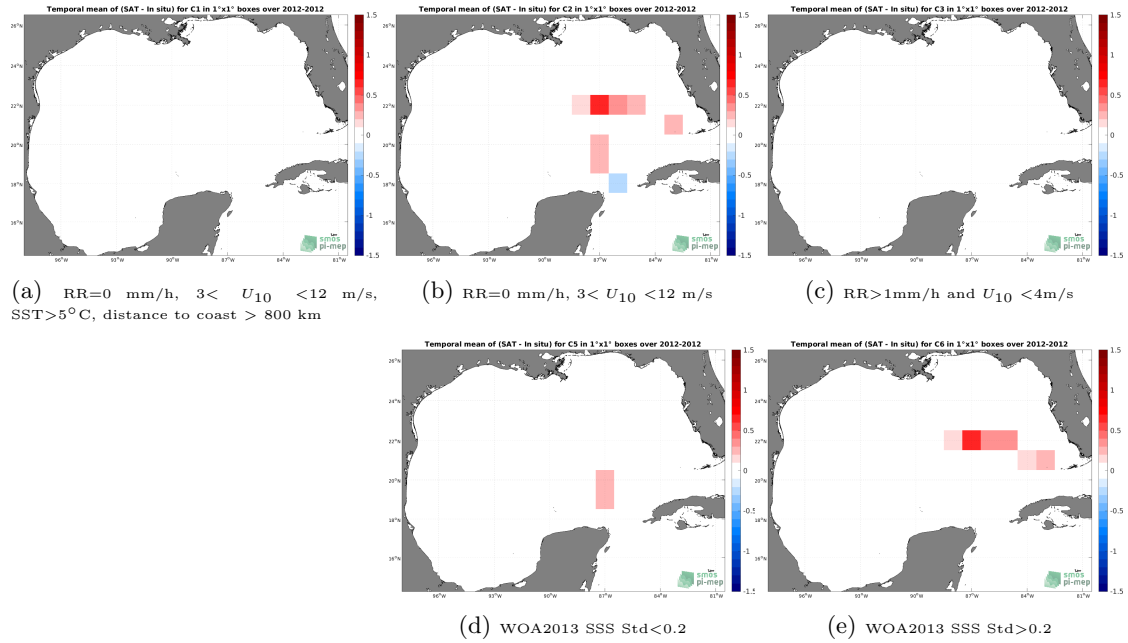
Figure 12: Temporal mean gridded over spatial boxes of size 1^{\circ}\times 1^{\circ} of \Delta SSS (Aquarius SSS L3 OR v5 - 7-Day running - Rain mask (NASA-GSFC) - TSG (GOSUD-Sailing-ship)) for 5 different subdatasets corresponding to:RR=0 mm/h, 3 < U_{10} < 12 m/s, SST >5^{\circ}\text{C} , distance to coast > 800 km (a), RR=0 mm/h, 3 < U_{10} < 12 m/s (b), RR >1 mm/h and U_{10} < 4 m/s (c), WOA2013 SSS Std <0.2 (d), WOA2013 SSS Std >0.2 (e).
