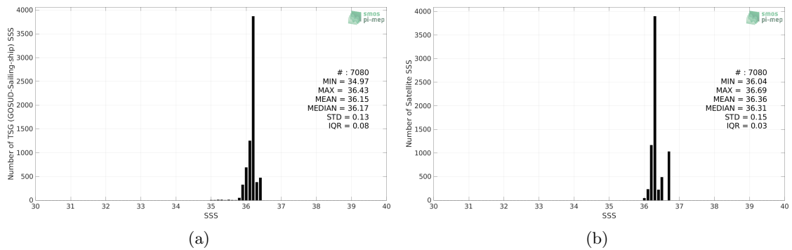
Figure 2: Histograms of SSS from TSG (GOSUD-Sailing-ship) (a) and Aquarius SSS L3 OR v5 - 7-Day running - Rain mask (NASA-GSFC) (b) considering all match-up pairs per bins of 0.1 over the Gulf of Mexico Pi-MEP region and for the full satellite product period.
