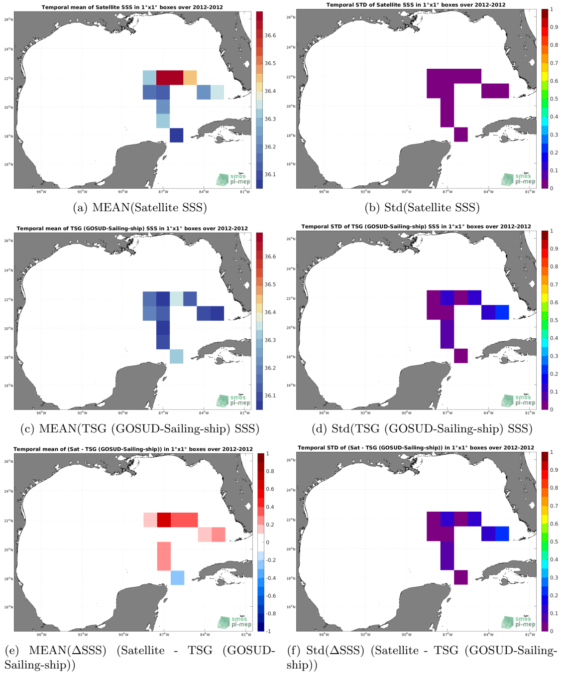
Figure 6: Temporal mean (left) and Std (right) of SSS from Aquarius SSS L3 OR v5 - 7-Day running - Rain mask (NASA-GSFC) (top), TSG (GOSUD-Sailing-ship) (middle), and of \Delta SSS (Satellite - TSG (GOSUD-Sailing-ship)). Only match-up pairs are used to generate these maps.
