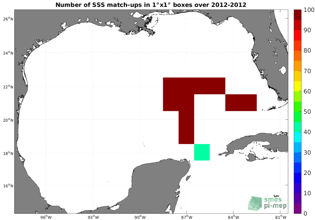
Figure 4: Number of SSS match-ups between TSG (GOSUD-Sailing-ship) SSS and the Aquarius SSS L3 OR v5 - 7-Day running - Rain mask (NASA-GSFC) SSS product for the Gulf of Mexico Pi-MEP region over 1^\circ \times 1^\circ boxes and for the full satellite product period.
