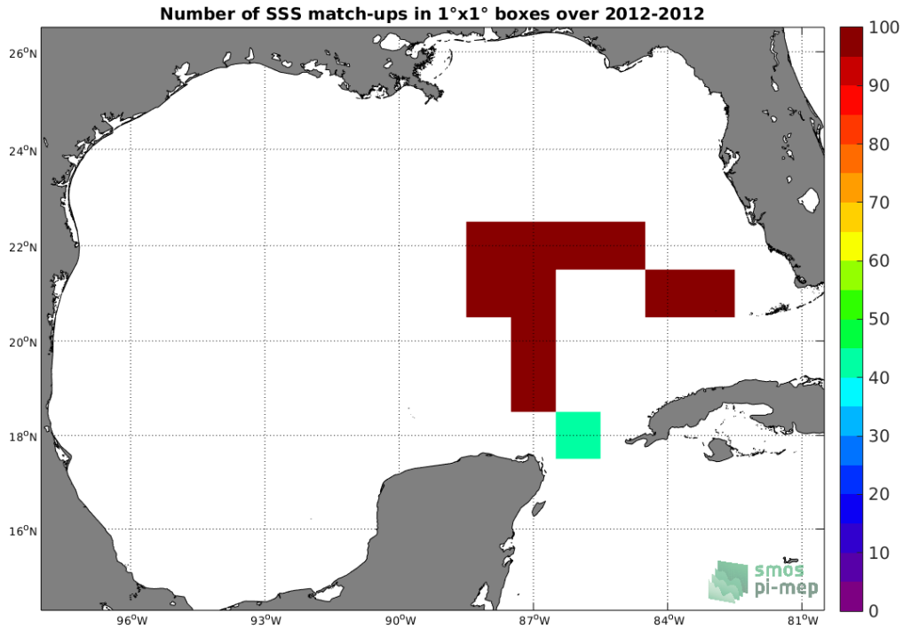
Figure 4: Number of SSS match-ups between TSG (GOSUD-Sailing-ship) SSS and the Aquarius SSS L3 OR v5 - 7-Day running - Rain mask (NASA-GSFC) SSS product for the Gulf of Mexico Pi-MEP region over 1^{\circ} \times 1^{\circ} boxes and for the full satellite product period.
