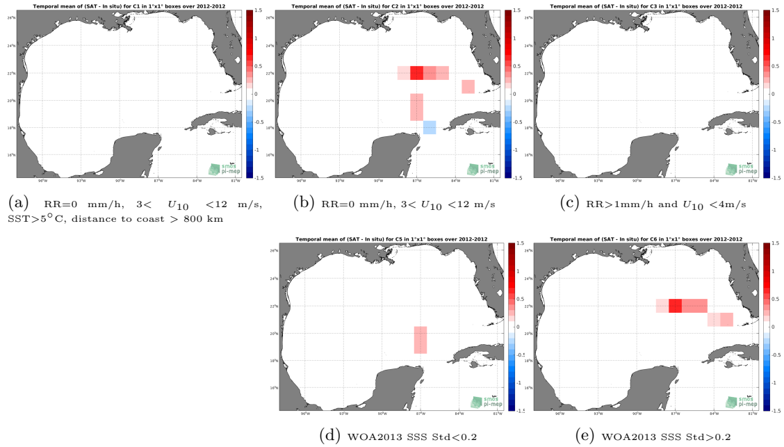
Figure 12: Temporal mean gridded over spatial boxes of size 1^\circ \times 1^\circ of \Delta SSS (Aquarius SSS L3 OR v5 - 7-Day running - Rain mask (NASA-GSFC) - TSG (GOSUD-Sailing-ship)) for 5 different subdatasets corresponding to:RR=0 mm/h, 3 < U_{10} < 12 m/s, SST >5^\circ\text{C} , distance to coast > 800 km (a), RR=0 mm/h, 3 < U_{10} < 12 m/s (b), RR >1 mm/h and U_{10} < 4 m/s (c), WOA2013 SSS Std <0.2 (d), WOA2013 SSS Std >0.2 (e).
