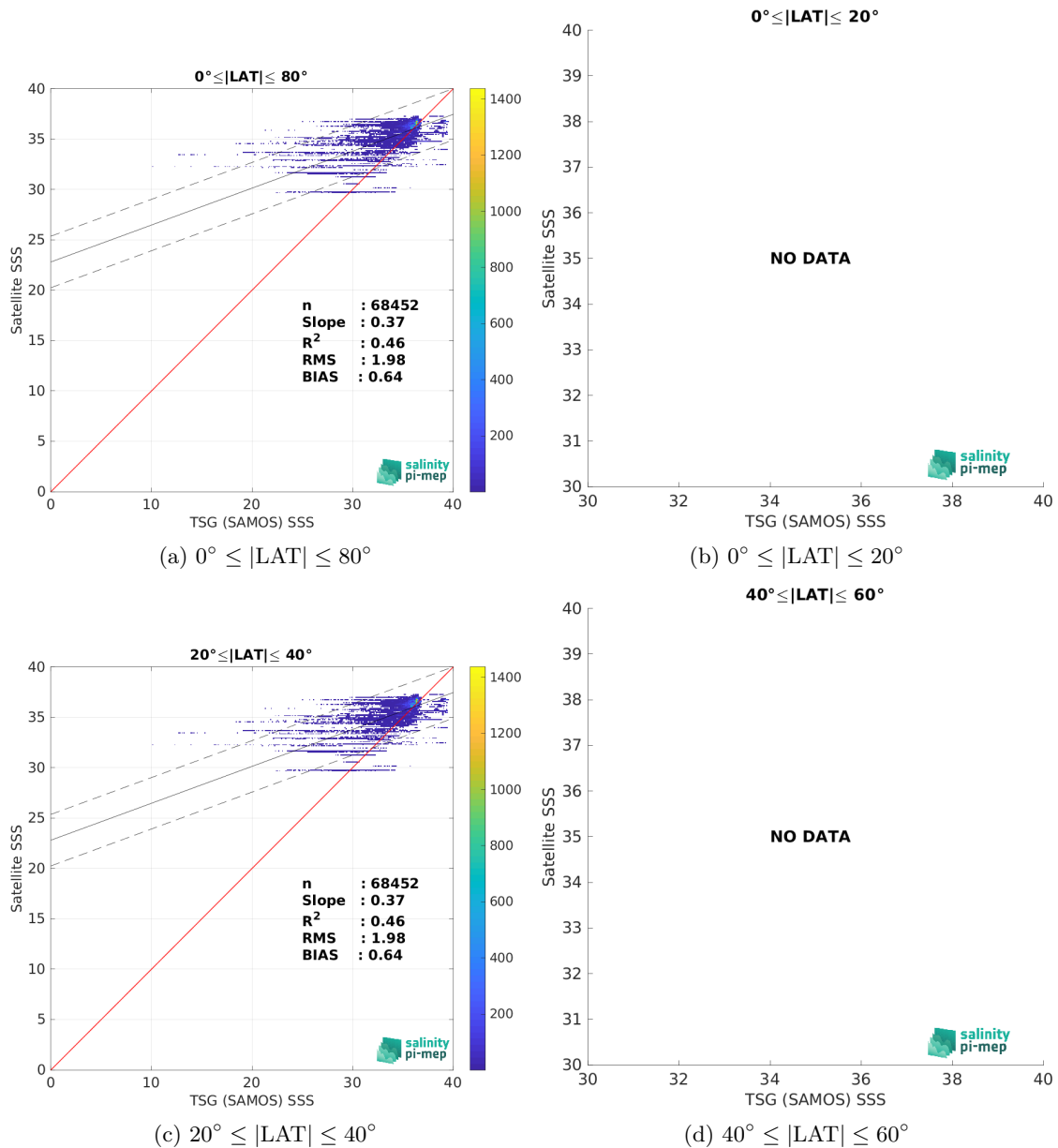
Figure 10: Contour maps of the concentration of Aquarius SSS L3 OR v5 - Monthly (NASA-GSFC) SSS (y-axis) versus TSG (SAMOS) SSS (x-axis) at match-up pairs for different latitude bands. For each plot, the red line shows x=y . The black thin and dashed lines indicate a linear fit through the data cloud and the \pm 95\% confidence levels, respectively. The number match-up pairs n , the slope and R^2 coefficient of the linear fit, the root mean square (RMS) and the mean bias between satellite and in situ data are indicated for each latitude band in each plots.
