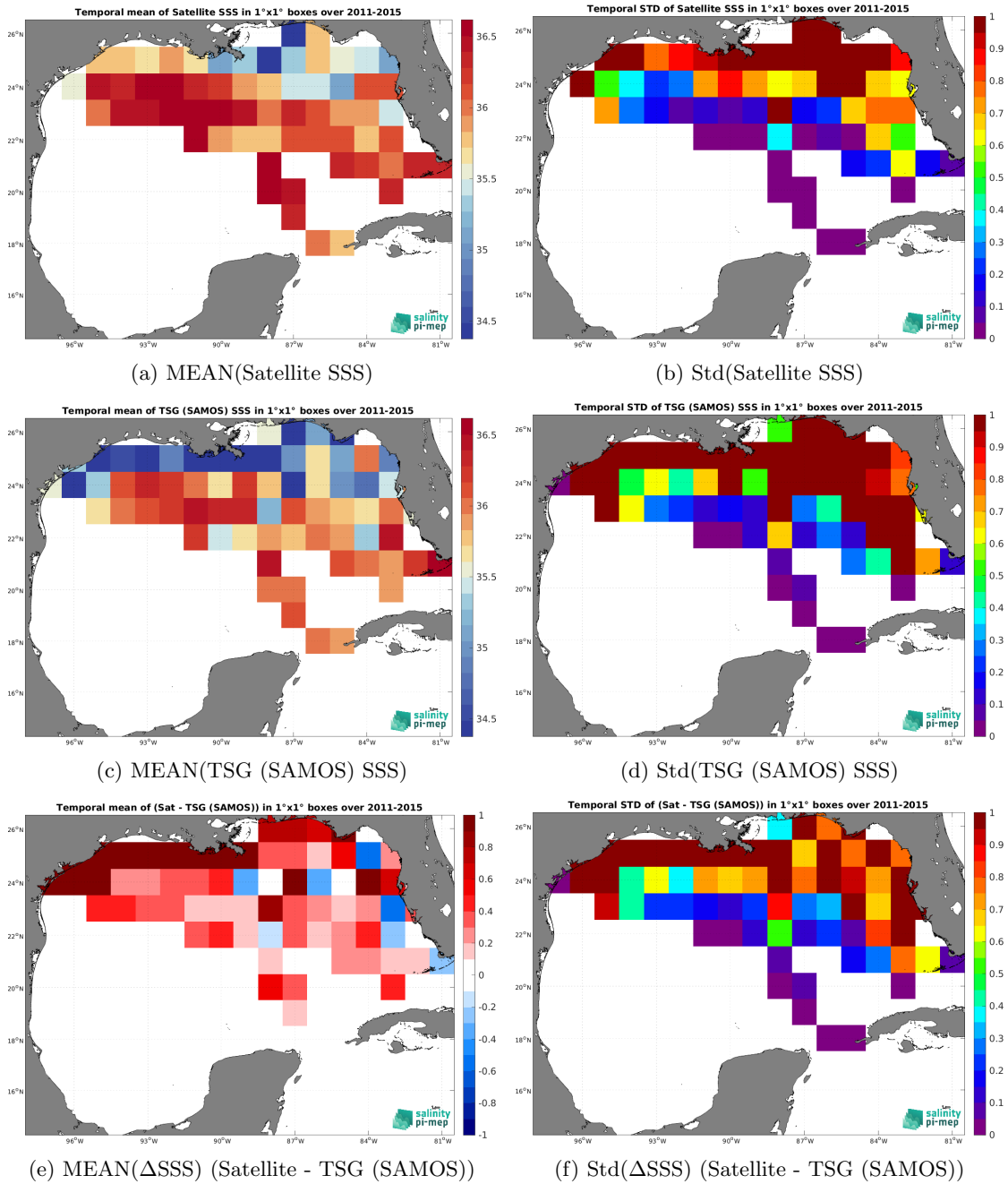
Figure 7: Temporal mean (left) and Std (right) of SSS from Aquarius SSS L3 OR v5 - Monthly (NASA-GSFC) (top), TSG (SAMOS) (middle), and of \Delta SSS (Satellite - TSG (SAMOS)). Only match-up pairs are used to generate these maps.
