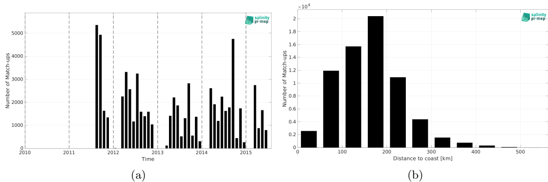
Figure 2: Number of match-ups between TSG (SAMOS) and Aquarius SSS L3 OR v5 - Monthly (NASA-GSFC) SSS as a function of time (a) and as function of the distance to coast (b) over the Gulf of Mexico Pi-MEP region and for the full satellite product period.
