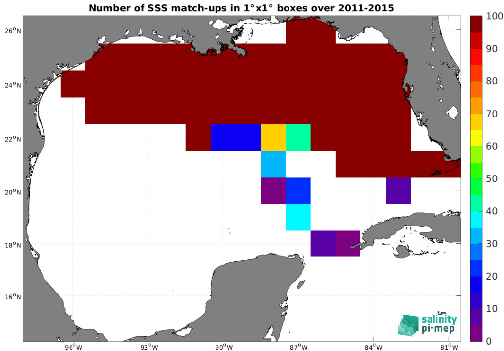
Figure 5: Number of SSS match-ups between TSG (SAMOS) SSS and the Aquarius SSS L3 OR v5 - Monthly (NASA-GSFC) SSS product for the Gulf of Mexico Pi-MEP region over 1^\circ \times 1^\circ boxes and for the full satellite product period.
