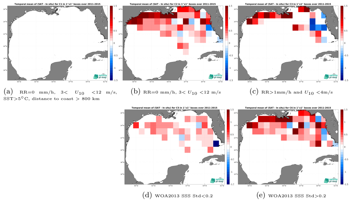
Figure 14: Temporal mean gridded over spatial boxes of size 1^\circ \times 1^\circ of \Delta SSS (Aquarius SSS L3 OR v5 - Monthly (NASA-GSFC) - TSG (SAMOS)) for 5 different subdatasets corresponding to:RR=0 mm/h, 3 < U_{10} < 12 m/s, SST >5^\circ C, distance to coast > 800 km (a), RR=0 mm/h, 3 < U_{10} < 12 m/s (b), RR >1 mm/h and U_{10} < 4 m/s (c), WOA2013 SSS Std <0.2 (d), WOA2013 SSS Std >0.2 (e).
