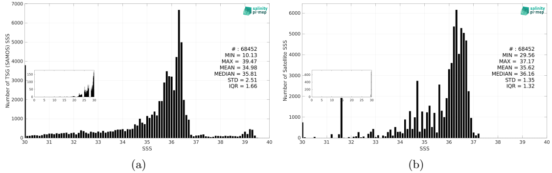
Figure 3: Histograms of SSS from TSG (SAMOS) (a) and Aquarius SSS L3 OR v5 - Monthly (NASA-GSFC) (b) considering all match-up pairs per bins of 0.1 over the Gulf of Mexico Pi-MEP region and for the full satellite product period.
