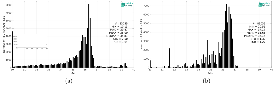
Figure 2: Histograms of SSS from TSG (SAMOS) (a) and Aquarius SSS L3 OR v5 - Monthly (NASA-GSFC) (b) considering all match-up pairs per bins of 0.1 over the Gulf of Mexico Pi-MEP region and for the full satellite product period.
