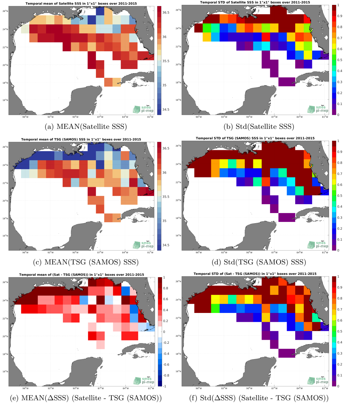
Figure 6: Temporal mean (left) and Std (right) of SSS from Aquarius SSS L3 OR v5 - Monthly (NASA-GSFC) (top), TSG (SAMOS) (middle), and of \Delta SSS (Satellite - TSG (SAMOS)). Only match-up pairs are used to generate these maps.
