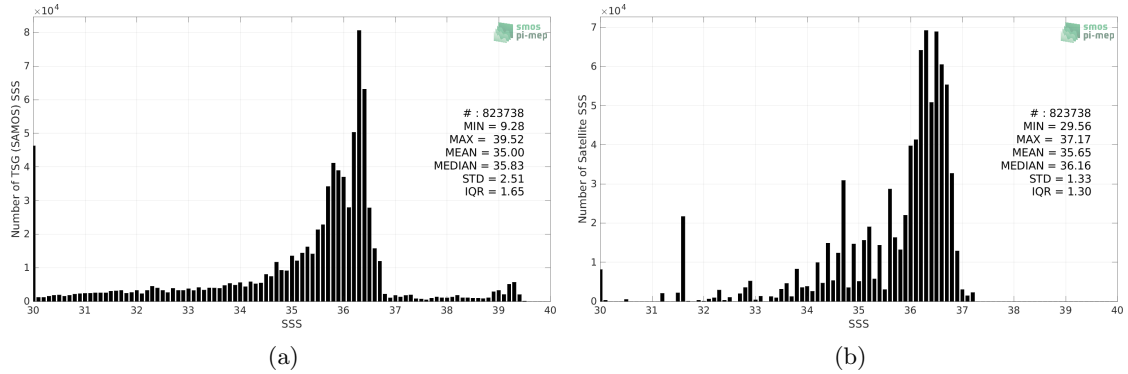
Figure 2: Histograms of SSS from TSG (SAMOS) (a) and Aquarius SSS L3 OR v5 - Monthly (NASA-GSFC) (b) considering all match-up pairs per bins of 0.1 over the Gulf of Mexico Pi-MEP region and for the full satellite product period.
