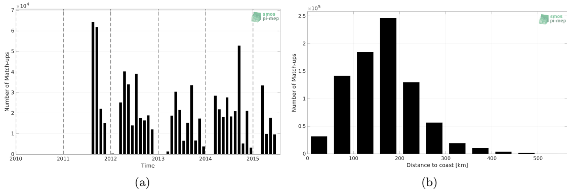
Figure 1: Number of match-ups between TSG (SAMOS) and Aquarius SSS L3 OR v5 - Monthly (NASA-GSFC) SSS as a function of time (a) and as function of the distance to coast (b) over the Gulf of Mexico Pi-MEP region and for the full satellite product period.
