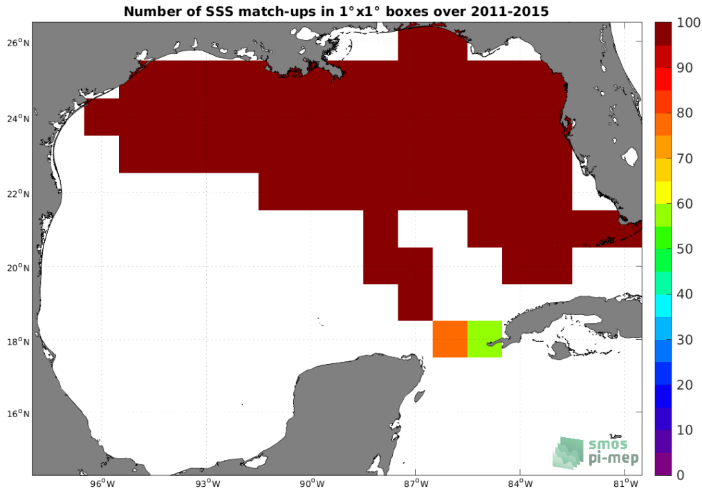
Figure 4: Number of SSS match-ups between TSG (SAMOS) SSS and the Aquarius SSS L3 OR v5 - Monthly (NASA-GSFC) SSS product for the Gulf of Mexico Pi-MEP region over 1^\circ \times 1^\circ boxes and for the full satellite product period.
