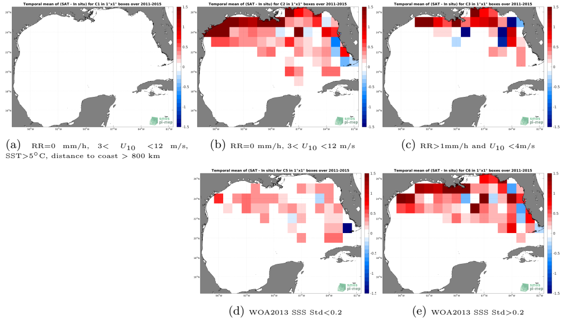
Figure 12: Temporal mean gridded over spatial boxes of size 1^{\circ}\times 1^{\circ} of \Delta\text{SSS} (Aquarius SSS L3 OR v5 - Monthly (NASA-GSFC) - TSG (SAMOS)) for 5 different subdatasets corresponding to:RR=0 mm/h, 3 < U_{10} < 12 m/s, SST >5^{\circ}\text{C} , distance to coast > 800 km (a), RR=0 mm/h, 3 < U_{10} < 12 m/s (b), RR >1 mm/h and U_{10} < 4 m/s (c), WOA2013 SSS Std <0.2 (d), WOA2013 SSS Std >0.2 (e).
