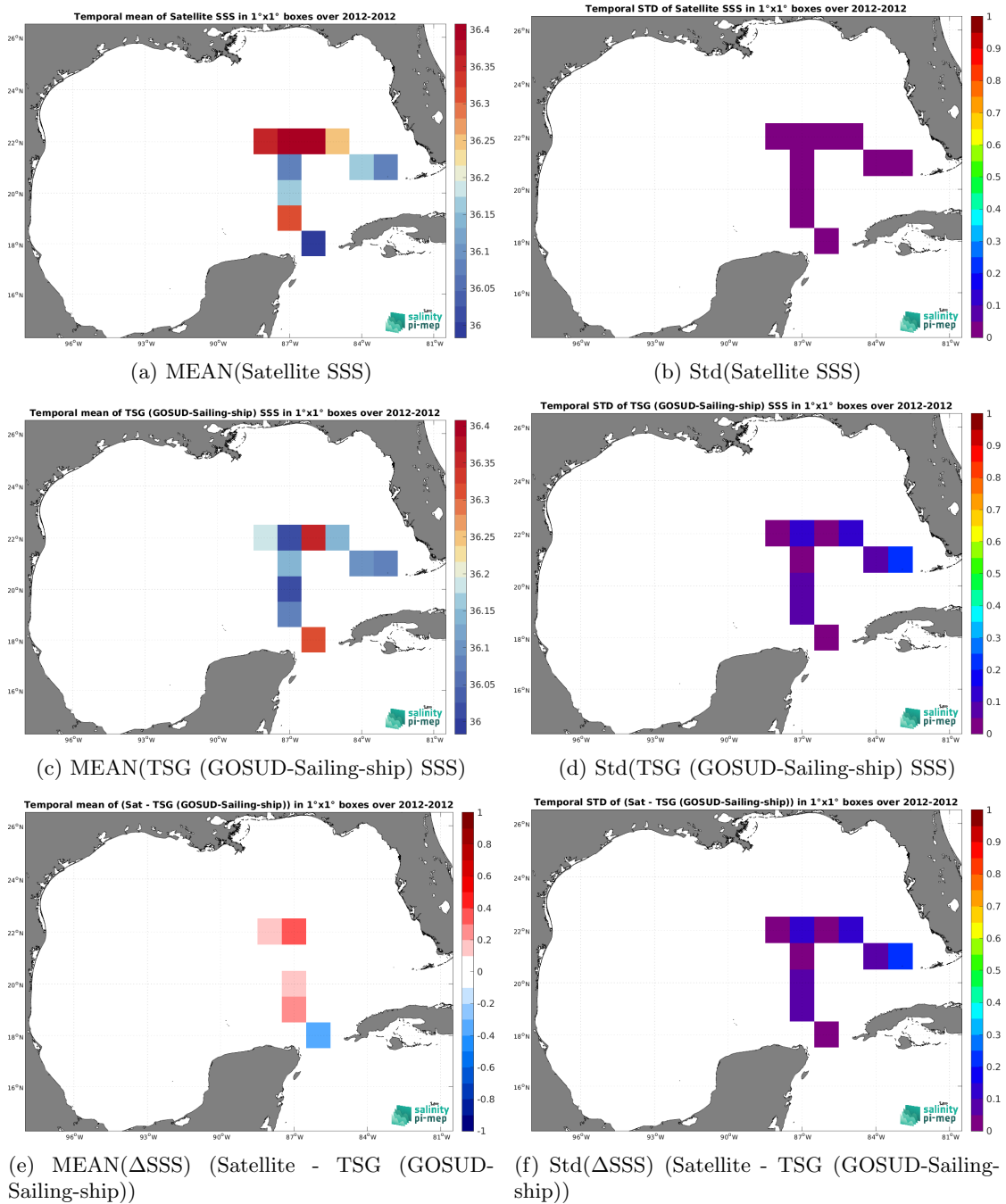
Figure 7: Temporal mean (left) and Std (right) of SSS from Aquarius SSS L3 OR v5 - Monthly (NASA-GSFC) (top), TSG (GOSUD-Sailing-ship) (middle), and of \Delta SSS (Satellite - TSG (GOSUD-Sailing-ship)). Only match-up pairs are used to generate these maps.
