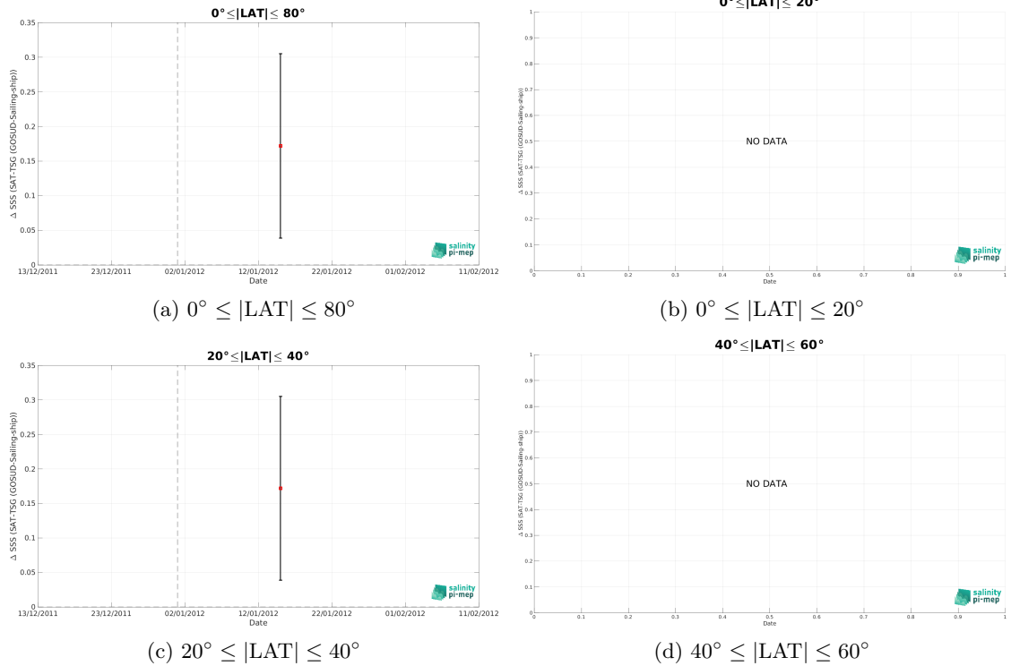
Figure 10: Monthly median (red curves) of \Delta SSS (Satellite - in situ TSG (GOSUD-Sailing-ship)) and \pm 1 Std (black vertical thick bars) as function of time for all the collected Pi-MEP match-up pairs estimated over the Gulf of Mexico Pi-MEP region and for the full satellite product period are shown for different latitude bands: (a) 80^\circ\text{S}-80^\circ\text{N} , (b) 20^\circ\text{S}-20^\circ\text{N} , (c) 40^\circ\text{S}-20^\circ\text{S} and 20^\circ\text{N}-40^\circ\text{N} and (d) 60^\circ\text{S}-40^\circ\text{S} and 40^\circ\text{N}-60^\circ\text{N} .
