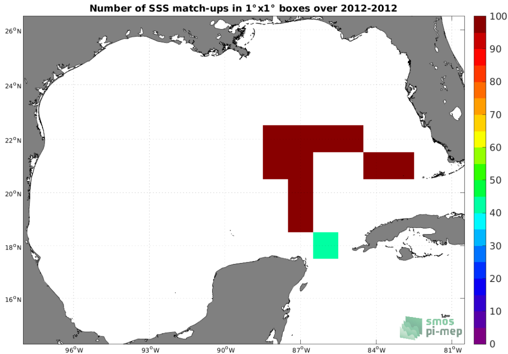
Figure 4: Number of SSS match-ups between TSG (GOSUD-Sailing-ship) SSS and the Aquarius SSS L3 OR v5 - Monthly (NASA-GSFC) SSS product for the Gulf of Mexico Pi-MEP region over 1^\circ \times 1^\circ boxes and for the full satellite product period.
