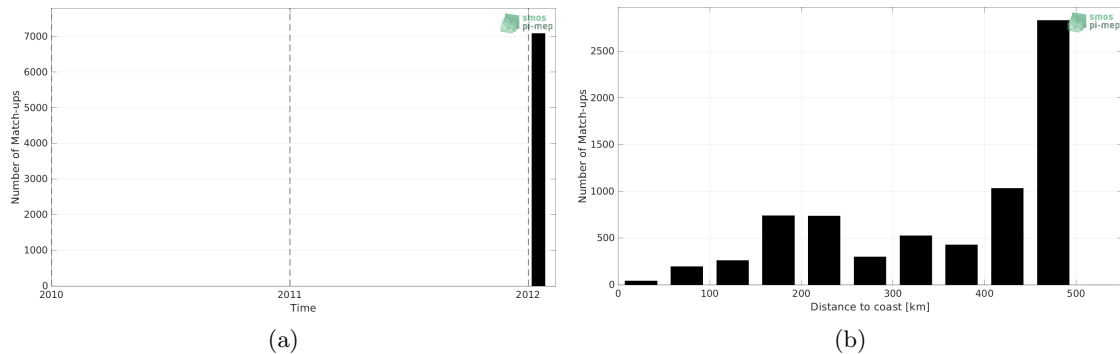
Figure 1: Number of match-ups between TSG (GOSUD-Sailing-ship) and Aquarius SSS L3 OR v5 - Monthly (NASA-GSFC) SSS as a function of time (a) and as function of the distance to coast (b) over the Gulf of Mexico Pi-MEP region and for the full satellite product period.
