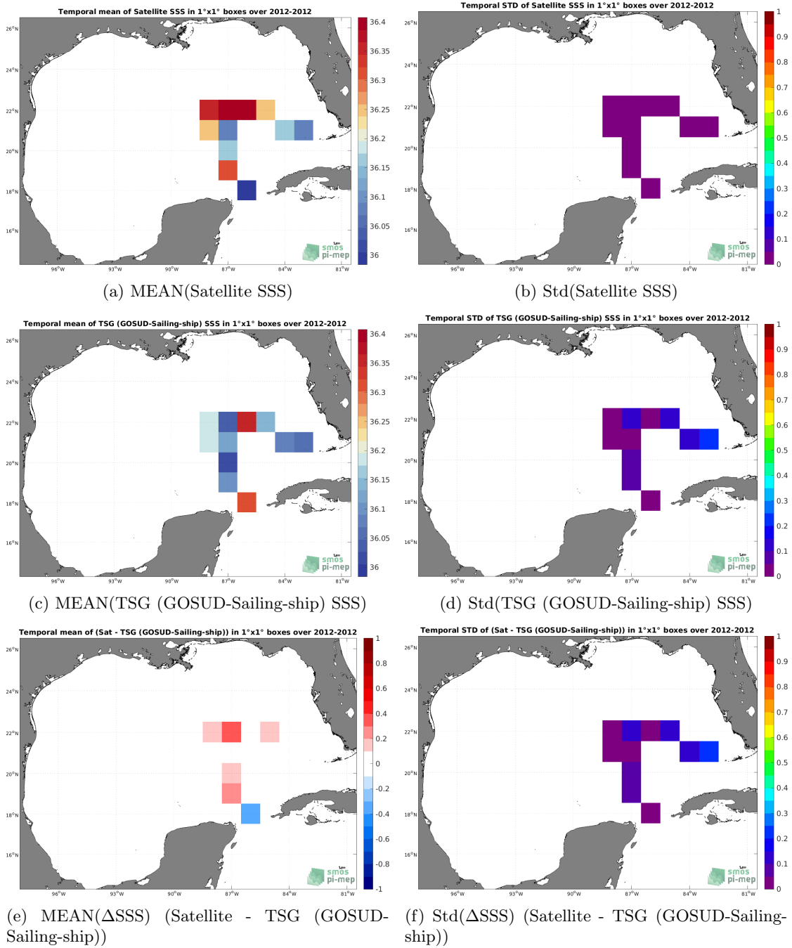
Figure 6: Temporal mean (left) and Std (right) of SSS from Aquarius SSS L3 OR v5 - Monthly (NASA-GSFC) (top), TSG (GOSUD-Sailing-ship) (middle), and of \Delta SSS (Satellite - TSG (GOSUD-Sailing-ship)). Only match-up pairs are used to generate these maps.
