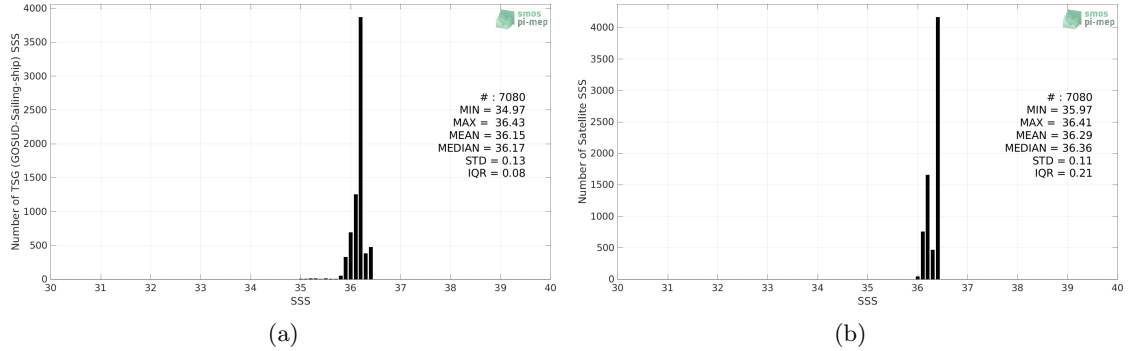
Figure 2: Histograms of SSS from TSG (GOSUD-Sailing-ship) (a) and Aquarius SSS L3 OR v5 - Monthly (NASA-GSFC) (b) considering all match-up pairs per bins of 0.1 over the Gulf of Mexico Pi-MEP region and for the full satellite product period.
