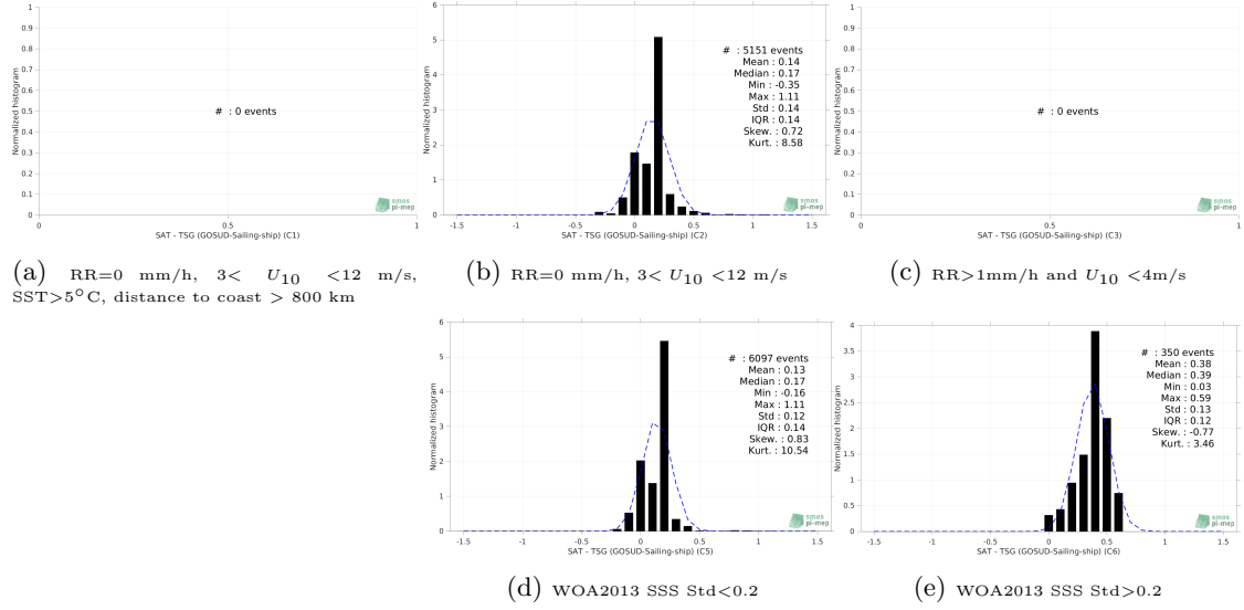
Figure 13: Normalized histogram of \Delta\text{SSS} (Aquarius SSS L3 OR v5 - Monthly (NASA-GSFC) - TSG (GOSUD-Sailing-ship)) for 5 different subdatasets corresponding to: RR=0 mm/h, 3 < U_{10} < 12 m/s, SST > 5^\circ\text{C} , distance to coast > 800 km (a), RR=0 mm/h, 3 < U_{10} < 12 m/s (b), RR > 1\text{mm/h} and U_{10} < 4\text{m/s} (c), WOA2013 SSS Std < 0.2 (d), WOA2013 SSS Std > 0.2 (e).
