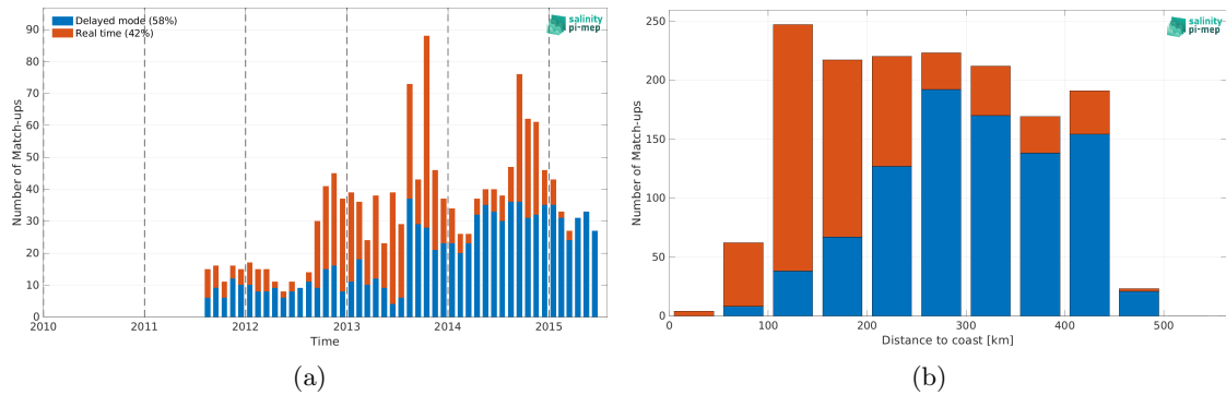
Figure 2: Number of match-ups between Argo and Aquarius SSS L3 OR v5 - Monthly (NASA-GSFC) SSS as a function of time (a) and as function of the distance to coast (b) over the Gulf of Mexico Pi-MEP region and for the full satellite product period.
