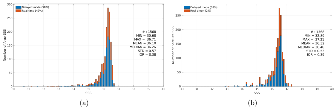
Figure 3: Histograms of SSS from Argo (a) and Aquarius SSS L3 OR v5 - Monthly (NASA-GSFC) (b) considering all match-up pairs per bins of 0.1 over the Gulf of Mexico Pi-MEP region and for the full satellite product period.
