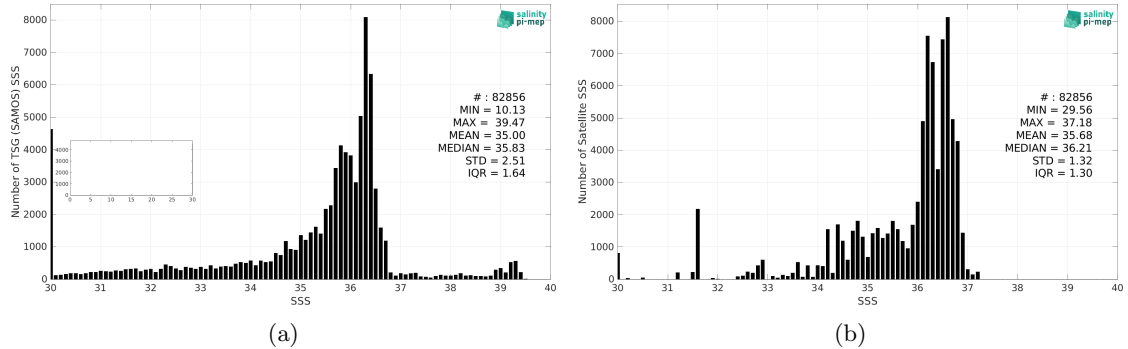
Figure 2: Histograms of SSS from TSG (SAMOS) (a) and Aquarius SSS L3 OR v5 - Monthly - Rain mask (NASA-GSFC) (b) considering all match-up pairs per bins of 0.1 over the Gulf of Mexico Pi-MEP region and for the full satellite product period.
