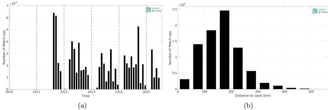
Figure 1: Number of match-ups between TSG (SAMOS) and Aquarius SSS L3 OR v5 - Monthly - Rain mask (NASA-GSFC) SSS as a function of time (a) and as function of the distance to coast (b) over the Gulf of Mexico Pi-MEP region and for the full satellite product period.
