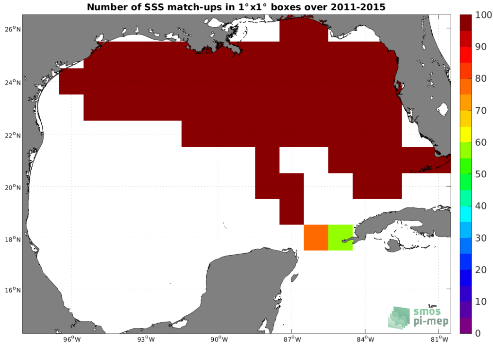
Figure 4: Number of SSS match-ups between TSG (SAMOS) SSS and the Aquarius SSS L3 OR v5 - Monthly - Rain mask (NASA-GSFC) SSS product for the Gulf of Mexico Pi-MEP region over 1^\circ \times 1^\circ boxes and for the full satellite product period.
