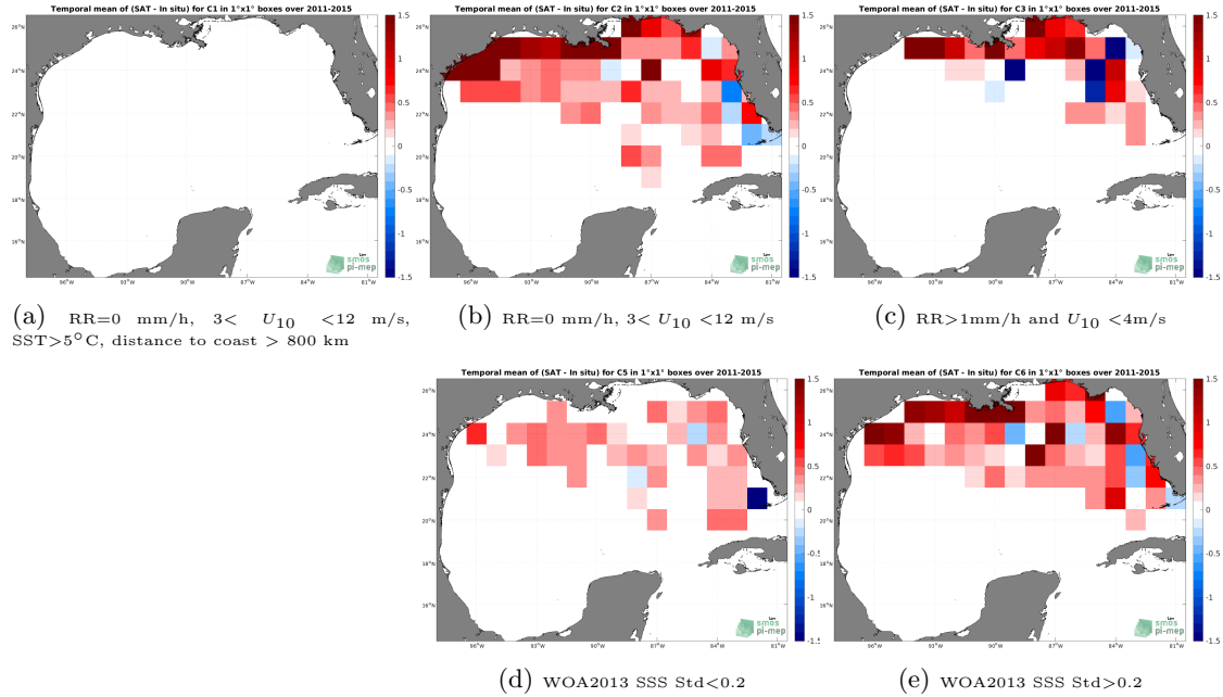
Figure 12: Temporal mean gridded over spatial boxes of size 1^{\circ}\times 1^{\circ} of \Delta\text{SSS} (Aquarius SSS L3 OR v5 - Monthly - Rain mask (NASA-GSFC) - TSG (SAMOS)) for 5 different subdatasets corresponding to:RR=0 mm/h, 3 < U_{10} < 12 m/s, SST >5^{\circ}\text{C} , distance to coast > 800 km (a), RR=0 mm/h, 3 < U_{10} < 12 m/s (b), RR >1 mm/h and U_{10} < 4 m/s (c), WOA2013 SSS Std <0.2 (d), WOA2013 SSS Std >0.2 (e).
