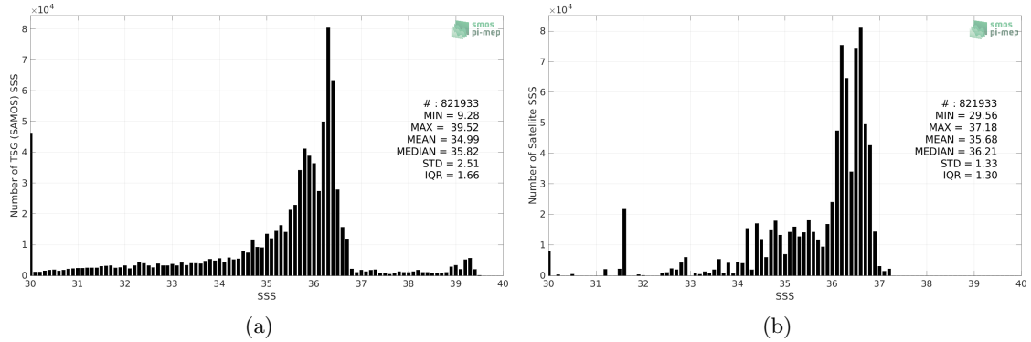
Figure 2: Histograms of SSS from TSG (SAMOS) (a) and Aquarius SSS L3 OR v5 - Monthly - Rain mask (NASA-GSFC) (b) considering all match-up pairs per bins of 0.1 over the Gulf of Mexico Pi-MEP region and for the full satellite product period.
