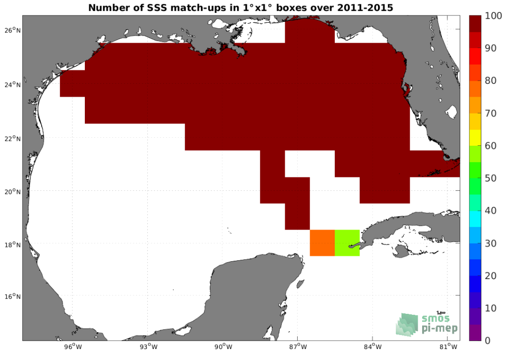
Figure 4: Number of SSS match-ups between TSG (SAMOS) SSS and the Aquarius SSS L3 OR v5 - Monthly - Rain mask (NASA-GSFC) SSS product for the Gulf of Mexico Pi-MEP region over 1^{\circ} \times 1^{\circ} boxes and for the full satellite product period.
